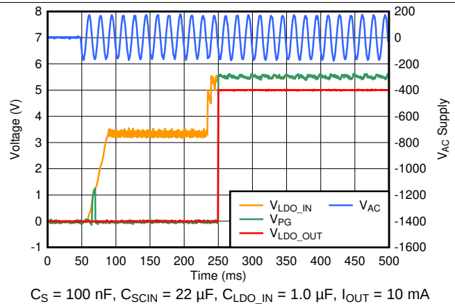
Figure 12. Slow Startup With the Minimum Required Cap-Drop Capacitor for 10-mA I_{OUT}
