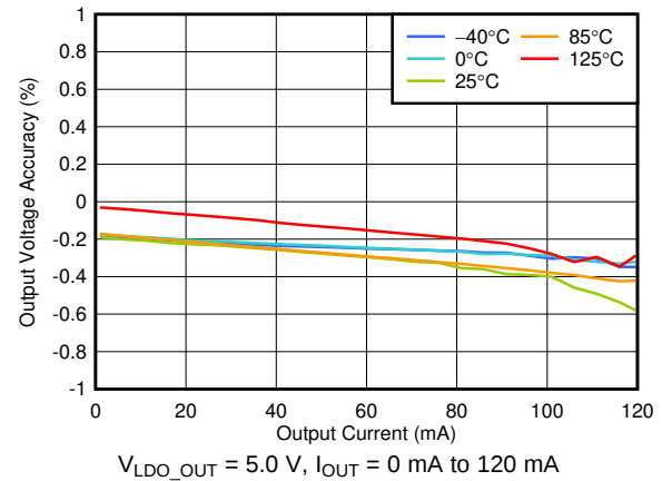
Figure 2. V_{LDO\_OUT} Accuracy vs I_{OUT}
