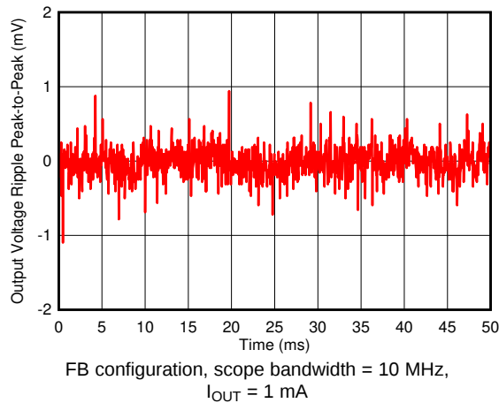
Figure 9. V_{LDO\_OUT} Ripple for FB Configuration
