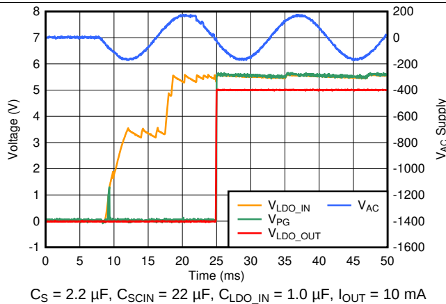
Figure 11. Fast Startup With Larger Than the Required Cap-Drop Capacitor for 10-mA I_{OUT}
