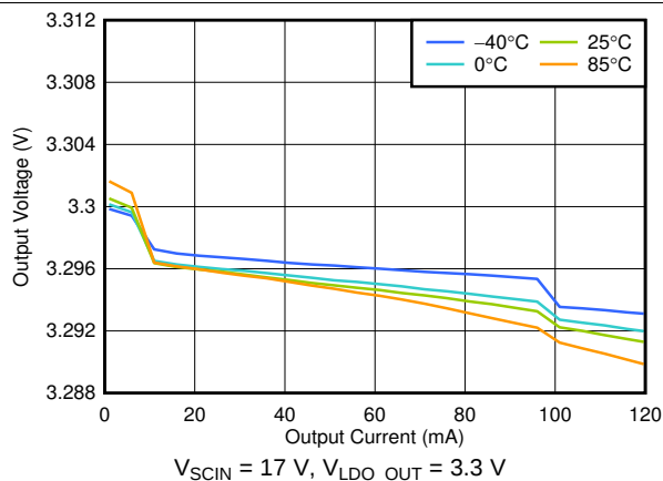
Figure 5. V_{LDO\_OUT} vs I_{OUT} DC Supply on the SCIN Pin
