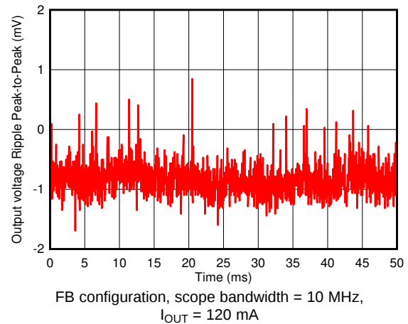
Figure 10. V_{LDO\_OUT} Ripple for FB Configuration
