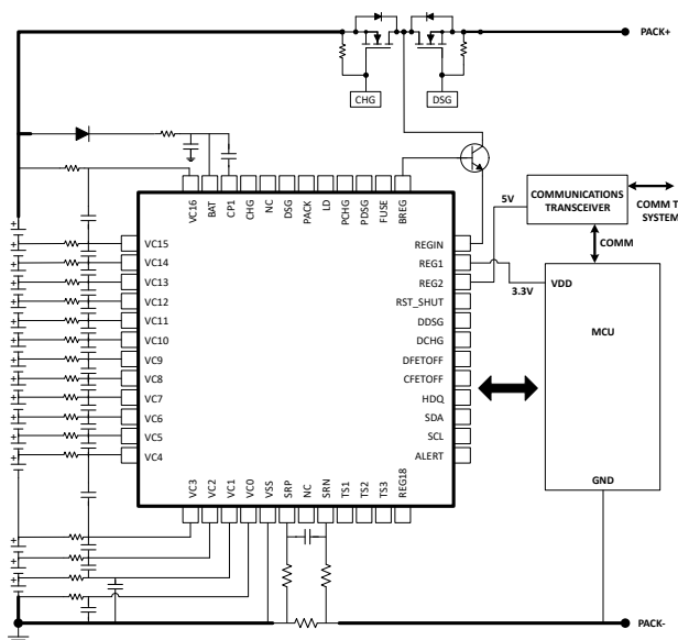
Simplified Schematic
