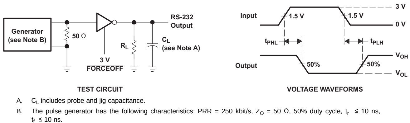
Figure 4. Driver Pulse Skew
