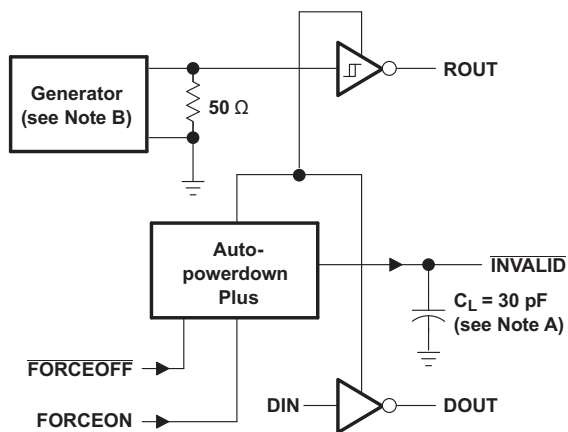
TEST CIRCUIT
