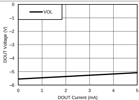
Figure 2. DOUT V_{OL} vs Load Current Other Drivers 3-k \Omega Load
