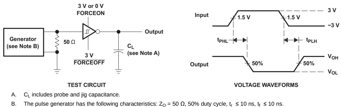
Figure 5. Receiver Propagation Delay Times
