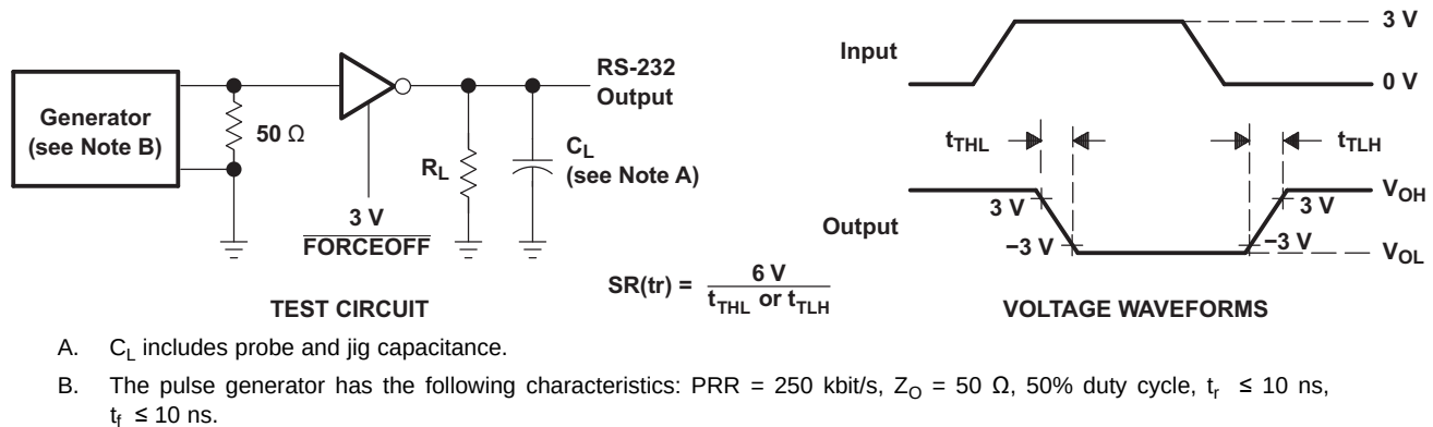
Figure 3. Driver Slew Rate
