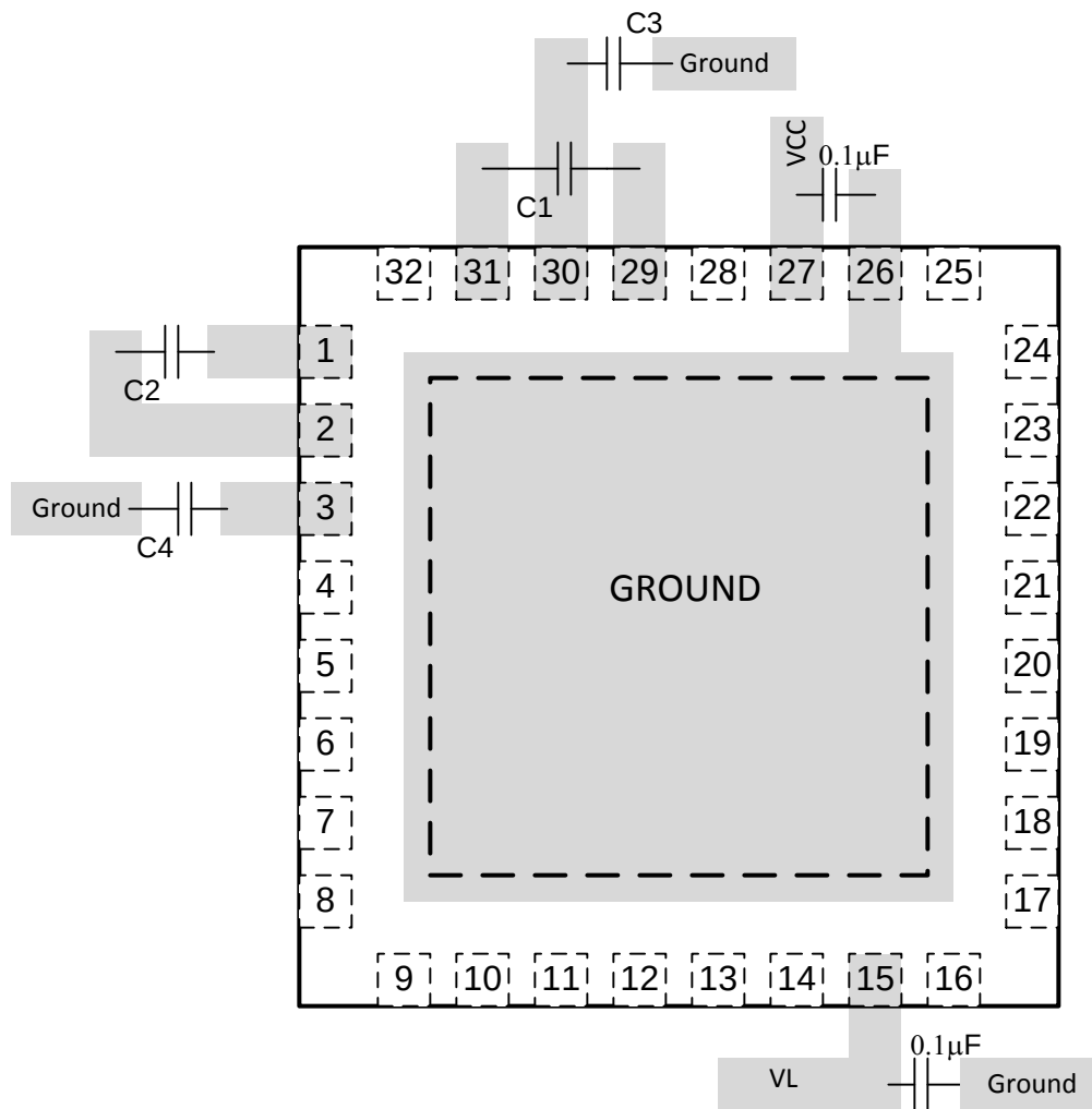
Figure 10. Layout Diagram
