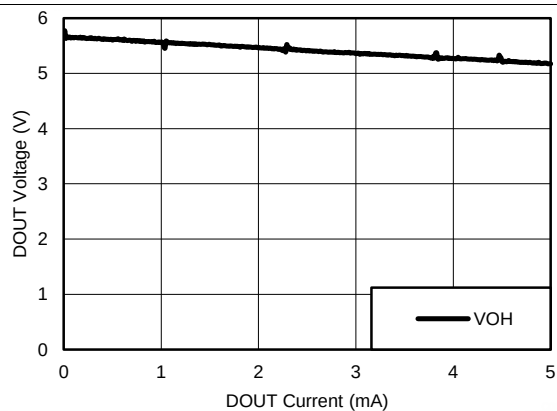
Figure 1. DOUT V_{OH} vs Load Current Other Drivers 3-k \Omega Load
