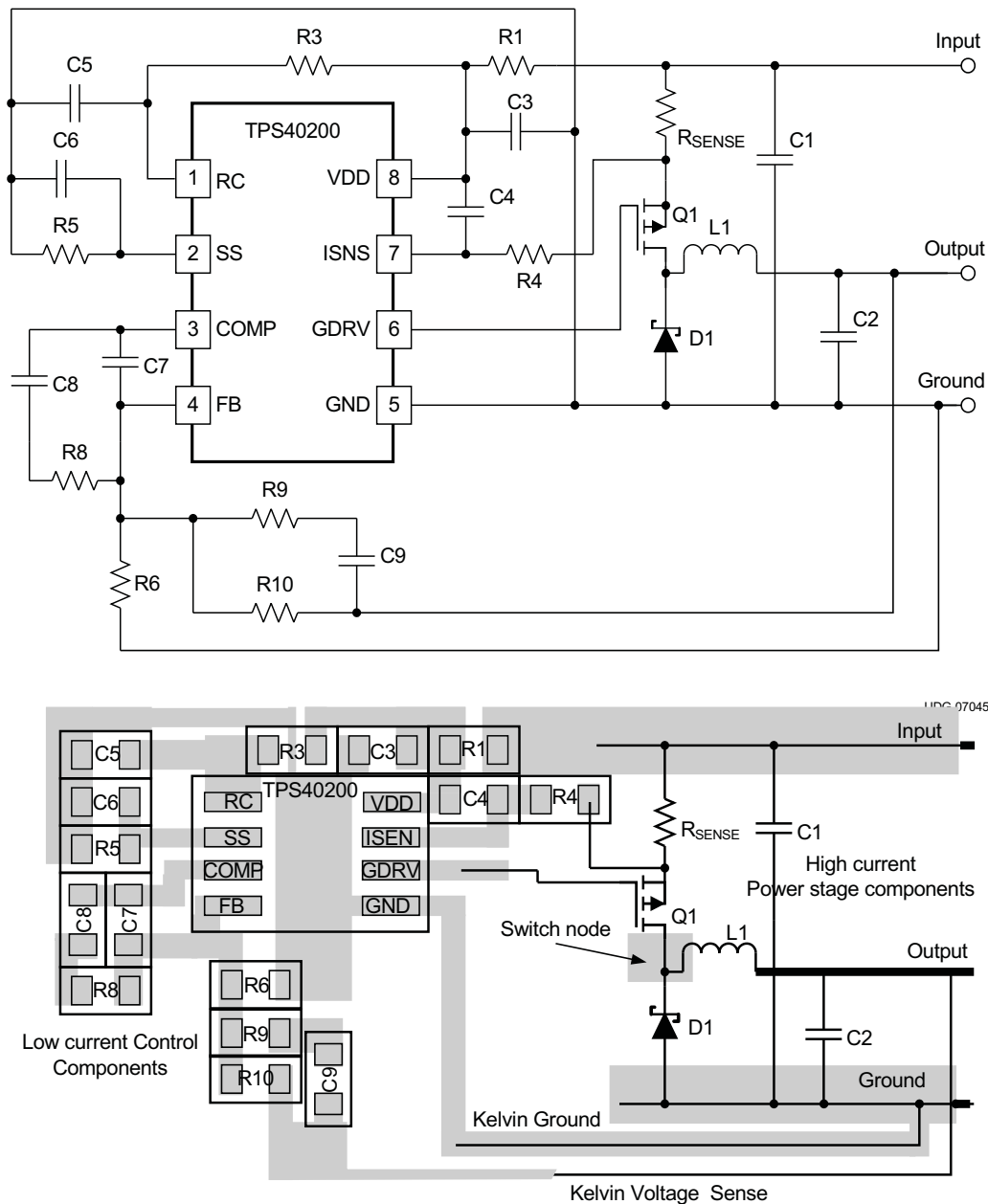
Figure 49. PC Board Layout Recommendations
