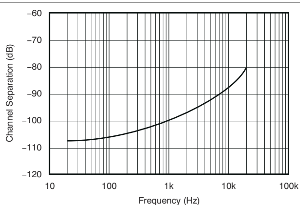
Figure 6-36. Channel Separation vs Frequency
