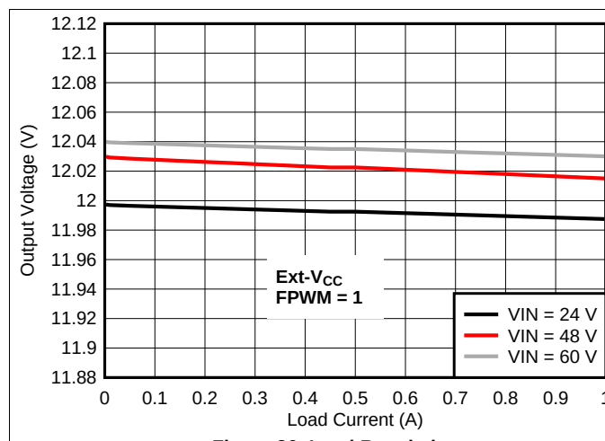
Figure 26. Load Regulation
