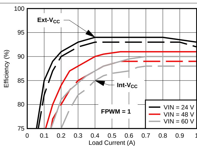
Figure 27. Efficiency vs I OUT (FPWM = 1)
