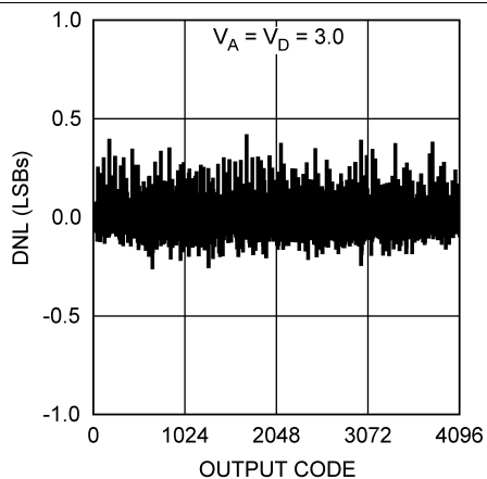
Figure 4. DNL
