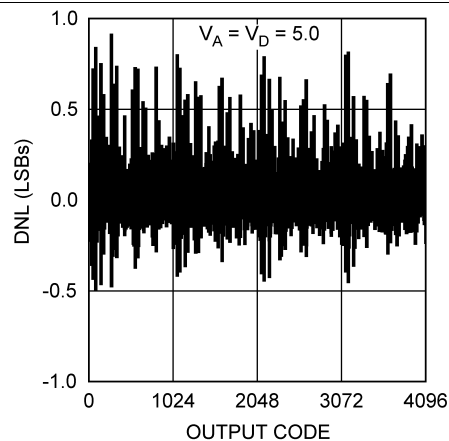
Figure 5. DNL
