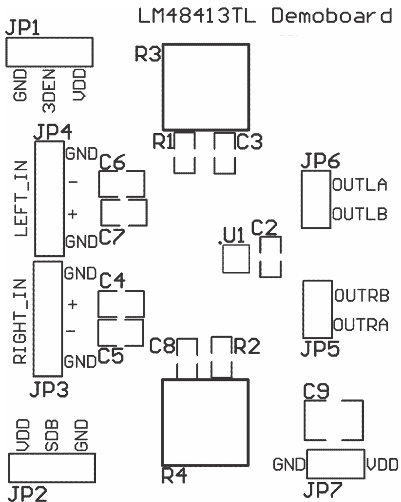
Figure 20. Top Silkscreen
