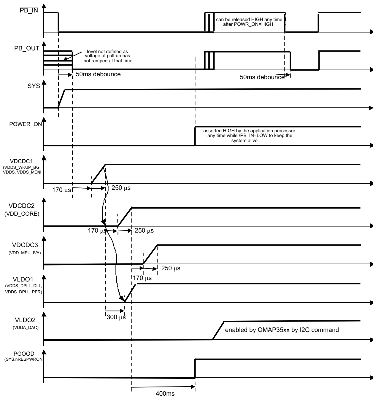
Figure 58. TPS650731: OMAP35xx timing
