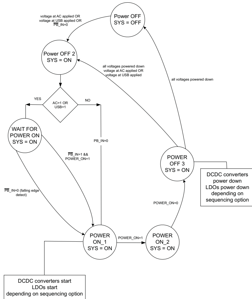
Figure 33. State Machine
