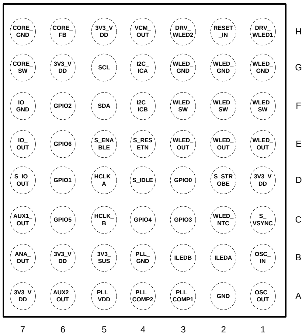
Pin Functions
