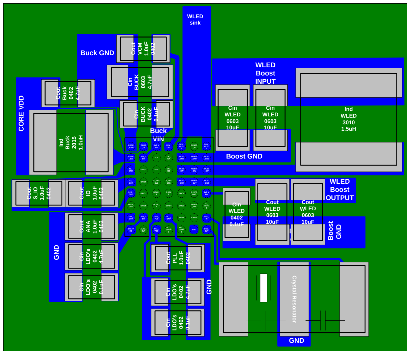
Figure 92. Layout
