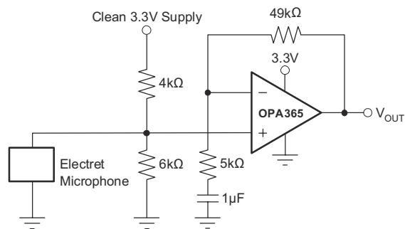
Figure 9-2. Microphone Preamplifier
