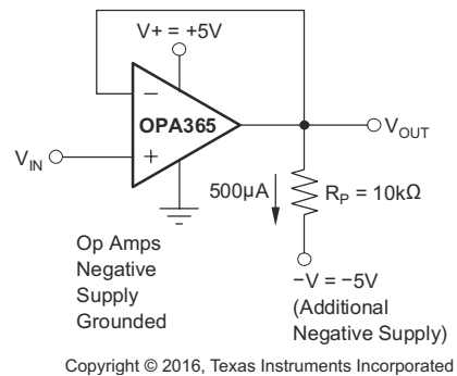
Figure 8-4. Swing-to-Ground
