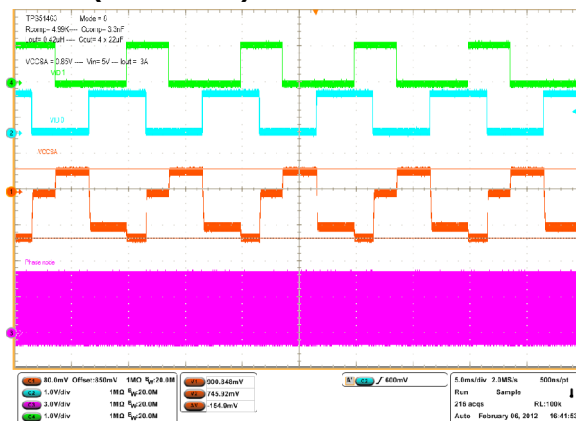
Figure 15. Mode=8, I_{OUT} = 3 A, VID Transienting
