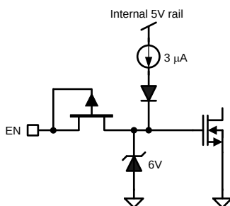
Figure 29. Enable Circuit
