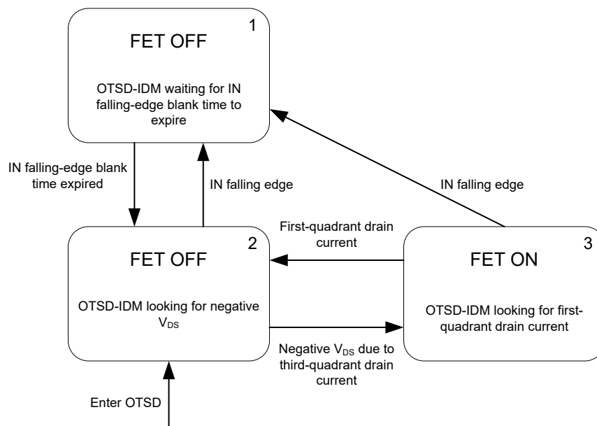
Figure 7-6. Overtemperature-Shutdown Ideal-Diode Mode (OTSD-IDM) State Machine
