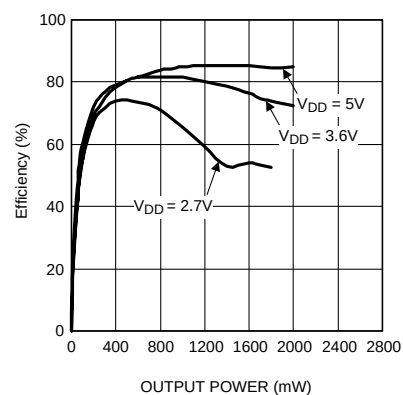
Efficiency vs Output Power R_L = 8\Omega , f = 1kHz
