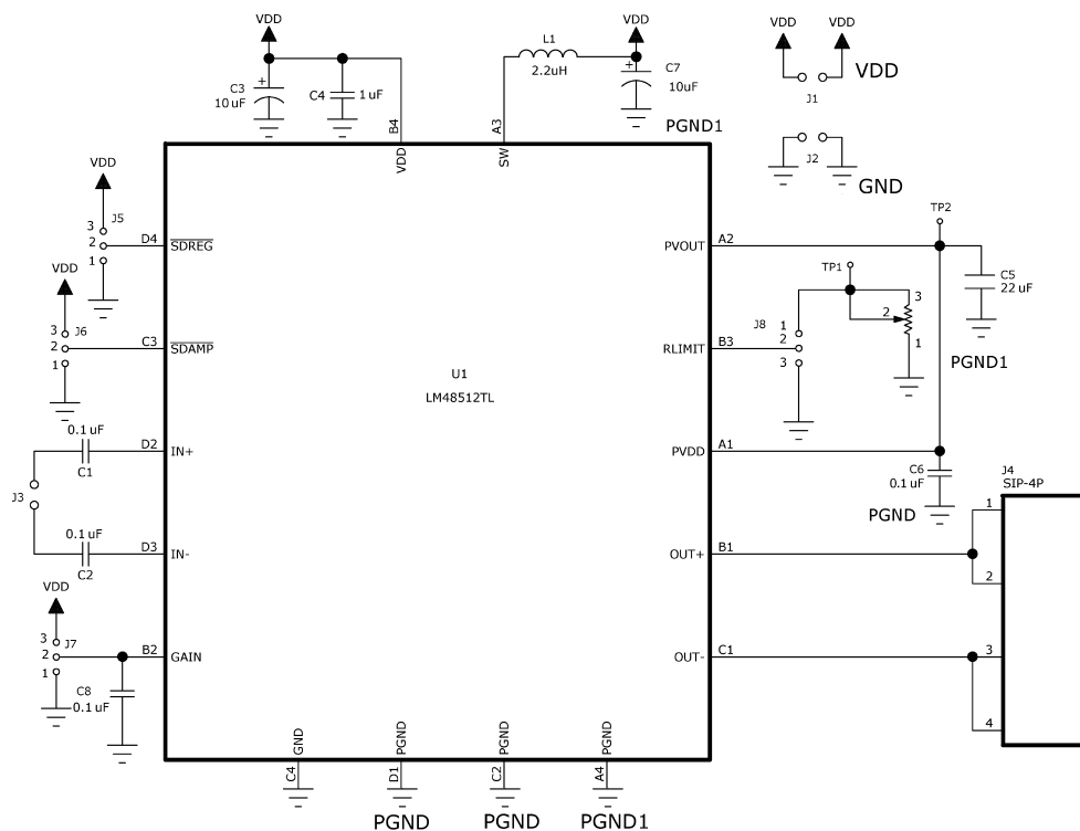
Figure 7. FIGURE 8. LM48512 Demo Board Schematic
