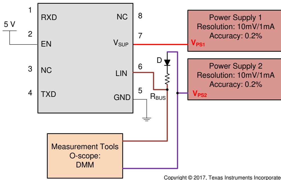
Figure 6-5. V_{SUP\_NON\_OP} Param 11
