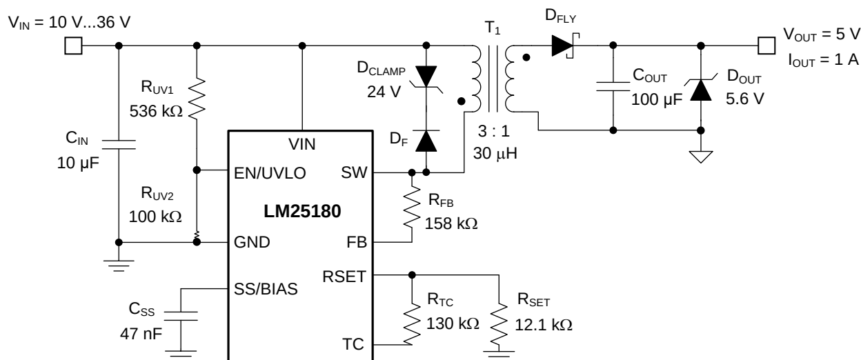
Figure 23. Schematic for Design 1 With V_{IN(nom)} = 24 V, V_{OUT} = 5 V, I_{OUT} = 1 A
