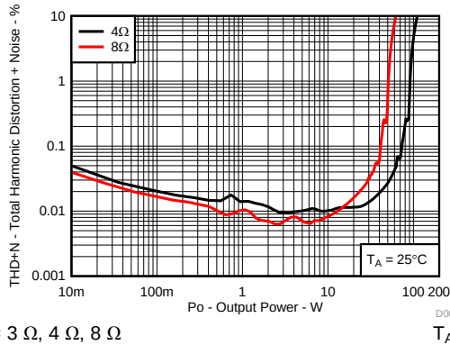
Figure 1. Total Harmonic Distortion + Noise vs Output Power, AD-mode
