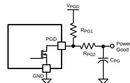
B) Long Delay at Rising Edge, Short Delay at Falling Edge
