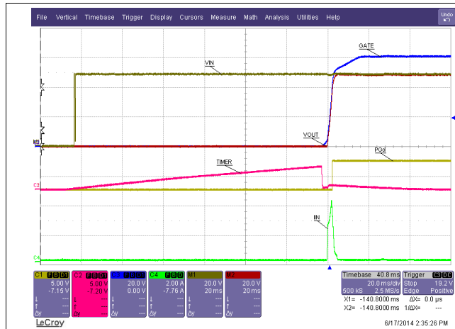
Figure 37. Insertion Delay
