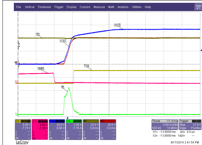
Figure 39. Start-Up V_{IN} = 40V
