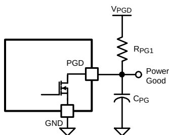
A) Delay at Rising Edge Only
