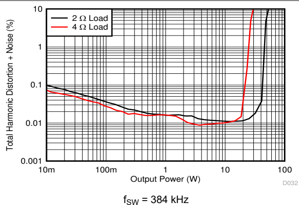
Figure 7-26. PBTL THD+N vs Power
