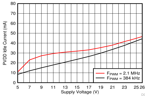
Figure 7-19. PVDD Idle Current vs Voltage
