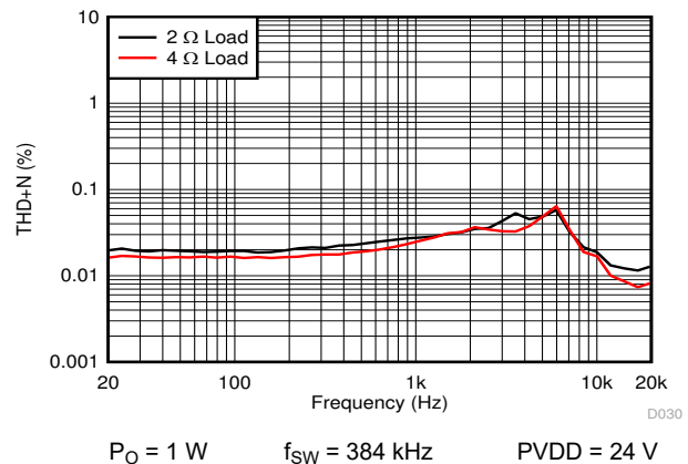
Figure 7-24. PBTL THD+N vs Frequency
