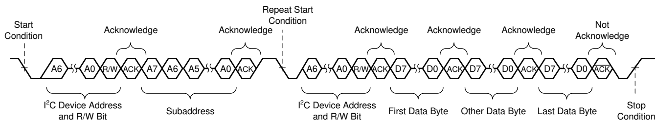
Figure 9-14. Sequential Read Transfer
