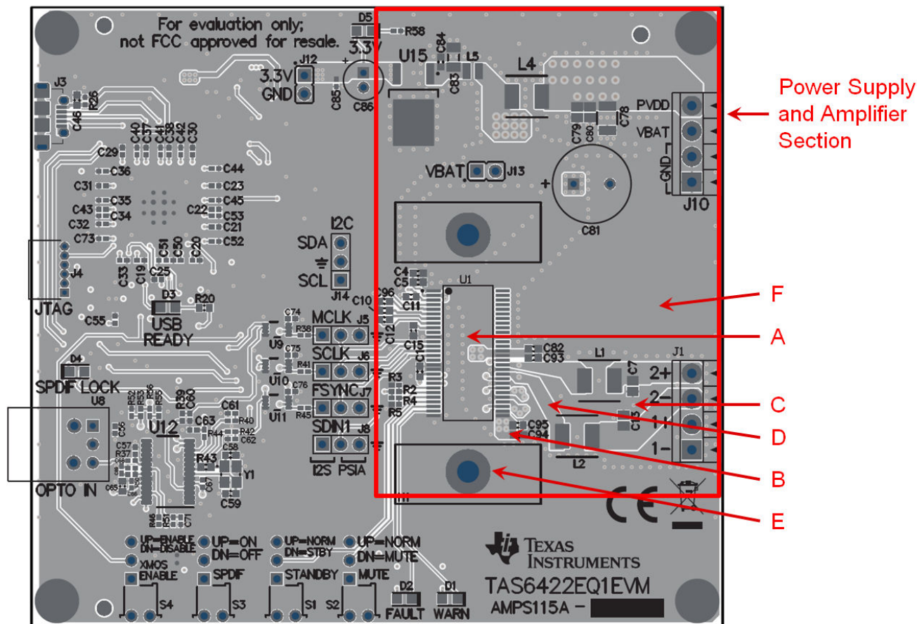
Figure 12-1. EVM Layout
