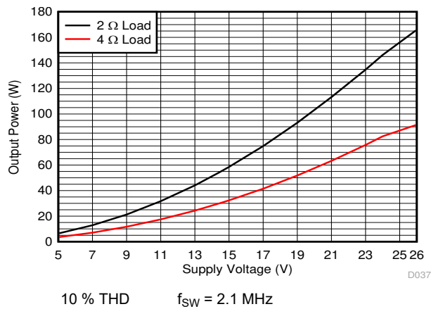
Figure 7-31. PBTL Output Power vs Voltage
