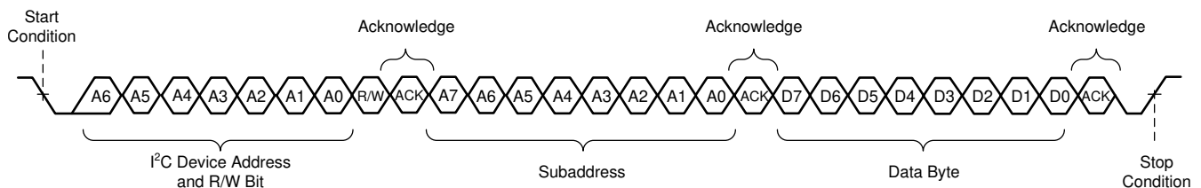
Figure 9-11. Random Write Transfer
