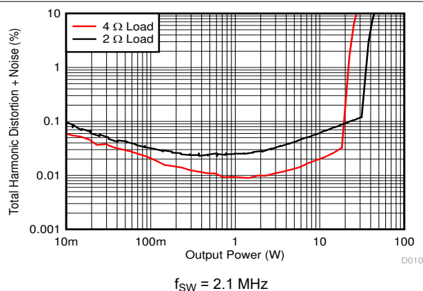
Figure 7-9. THD+N vs Power
