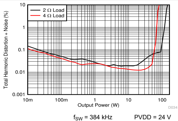
Figure 7-28. PBTL THD+N vs Power
