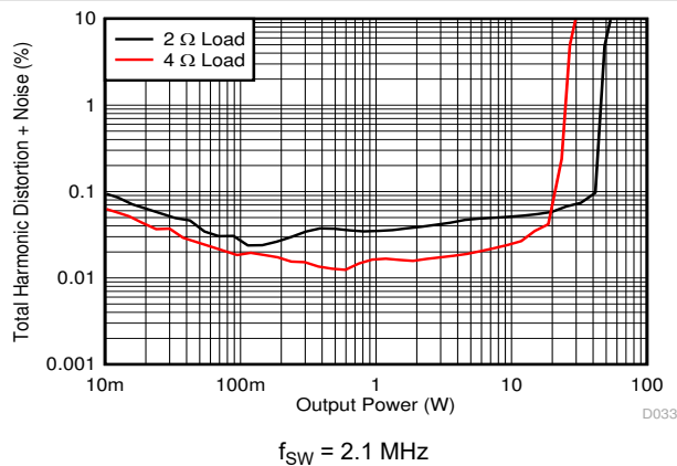
Figure 7-27. PBTL THD+N vs Power
