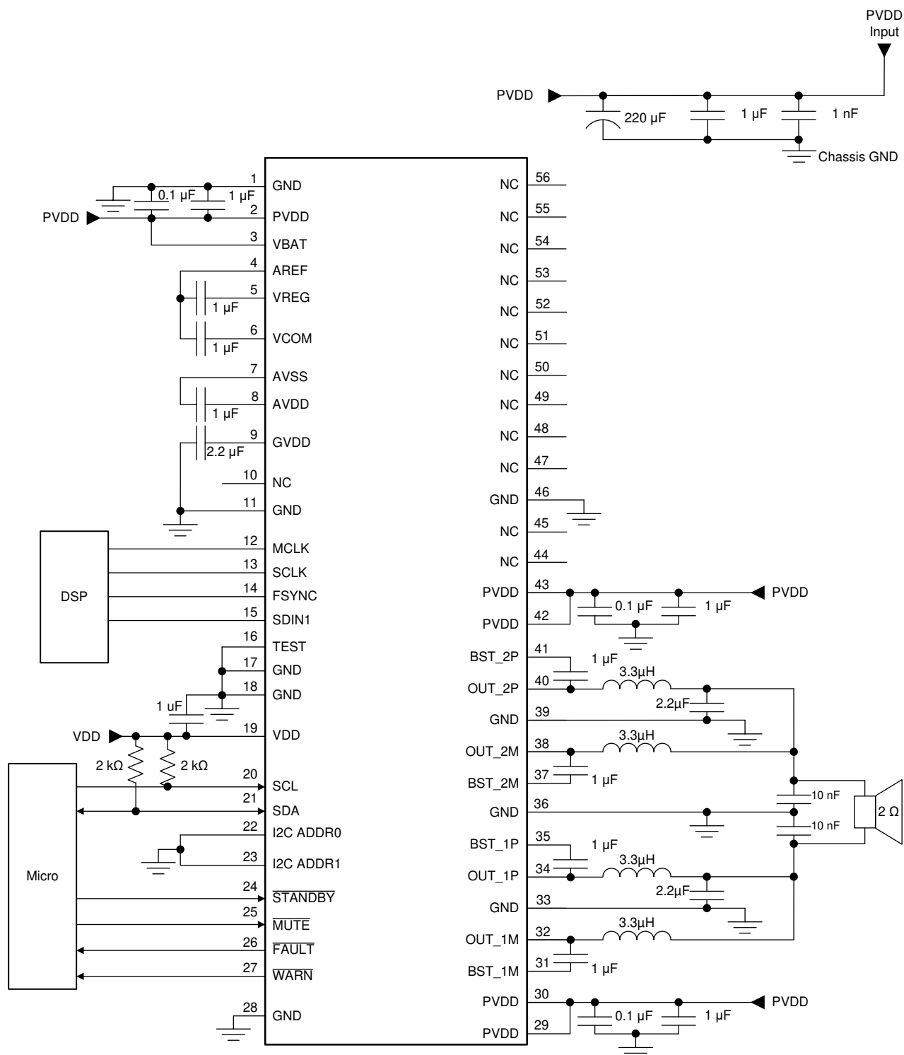
Figure 10-3. Typical 1-Channel PBTL Application Schematic
