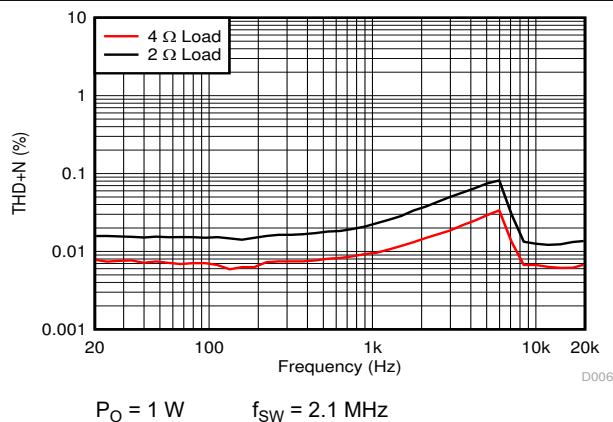
Figure 7-5. THD+N vs Frequency
