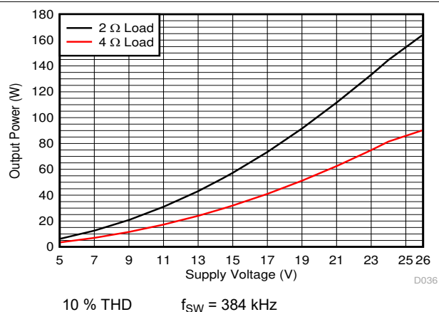
Figure 7-30. PBTL Output Power vs Voltage
