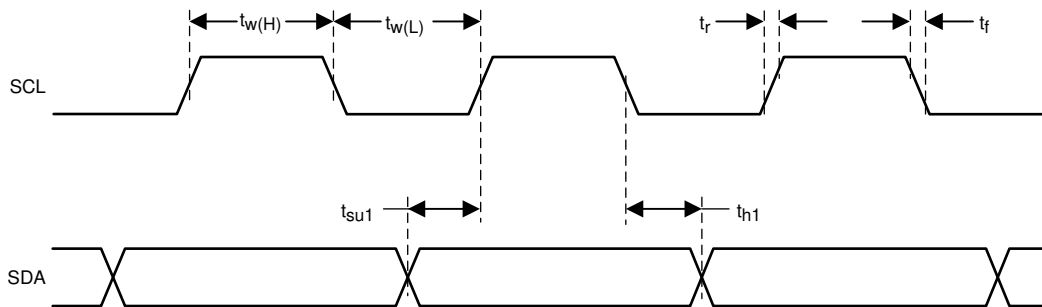
Figure 9-10. SCL and SDA Timing
