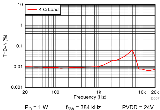
Figure 7-6. THD+N vs Frequency
