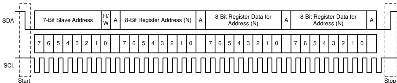
Figure 9-9. Typical I 2 C Sequence
