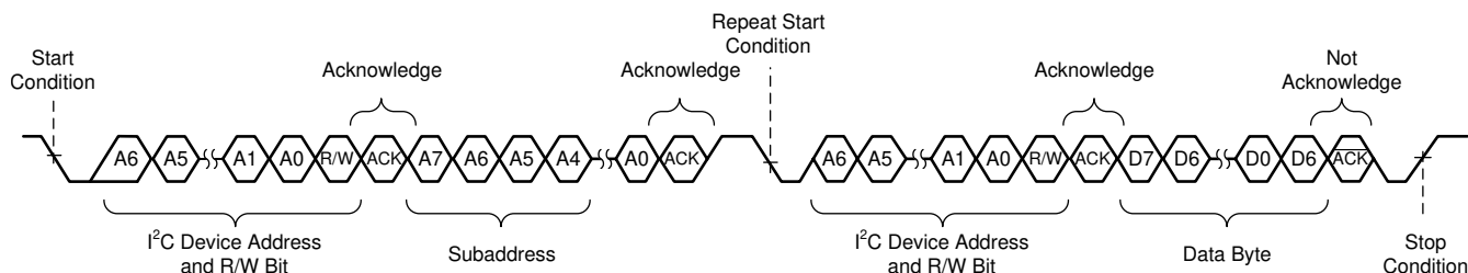
Figure 9-13. Random Read Transfer
