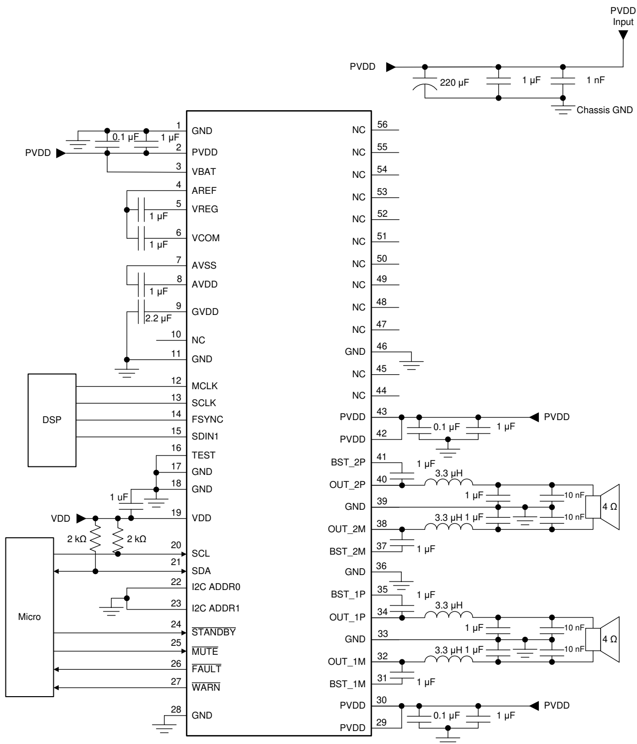
Figure 10-2. Typical 2-Channel BTL Application Schematic
