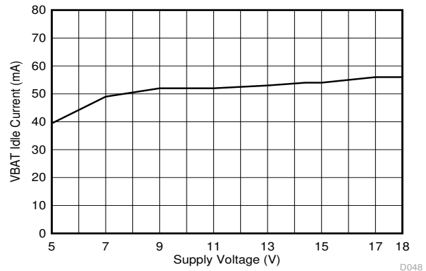
Figure 7-20. VBAT Idle Current vs Voltage
