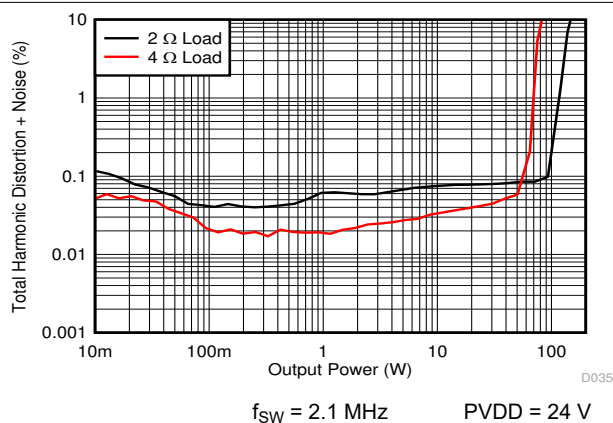
Figure 7-29. PBTL THD+N vs Power
