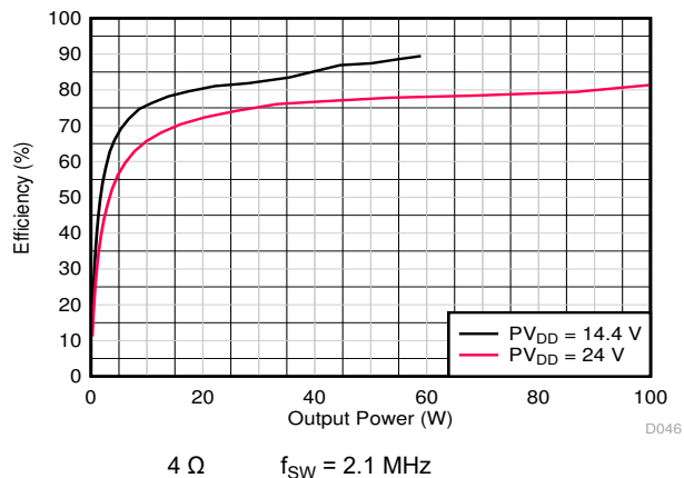
Figure 7-16. Power Efficiency vs Total Output Power
