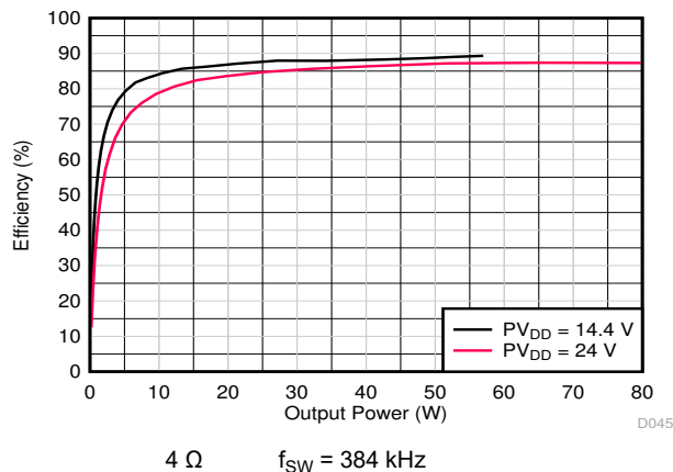
Figure 7-15. Power Efficiency vs Total Output Power
