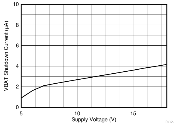
Figure 7-21. VBAT Standby Current vs Voltage
