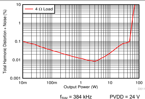
Figure 7-10. THD+N vs Power
