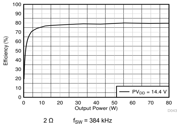
Figure 7-17. Power Efficiency vs Total Output Power
