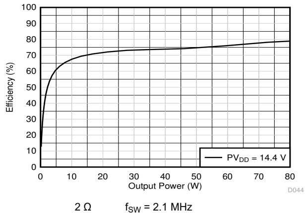
Figure 7-18. Power Efficiency vs Total Output Power
