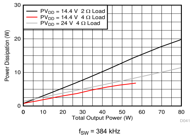
Figure 7-32. BTL Power Dissipation vs Total Output Power
