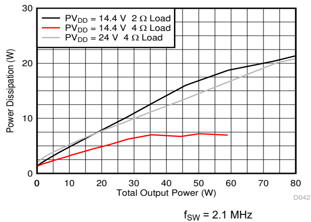
Figure 7-33. BTL Power Dissipation vs Total Output Power
