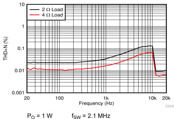
Figure 7-23. PBTL THD+N vs Frequency
