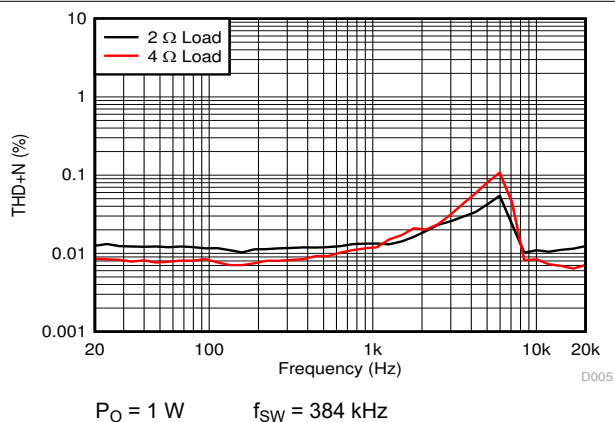
Figure 7-4. THD+N vs Frequency
