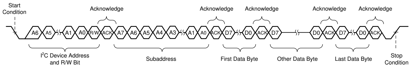
Figure 9-12. Sequential Write Transfer
