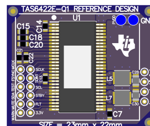
PCB AREA
