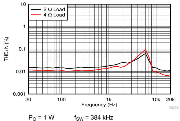
Figure 7-22. PBTL THD+N vs Frequency
