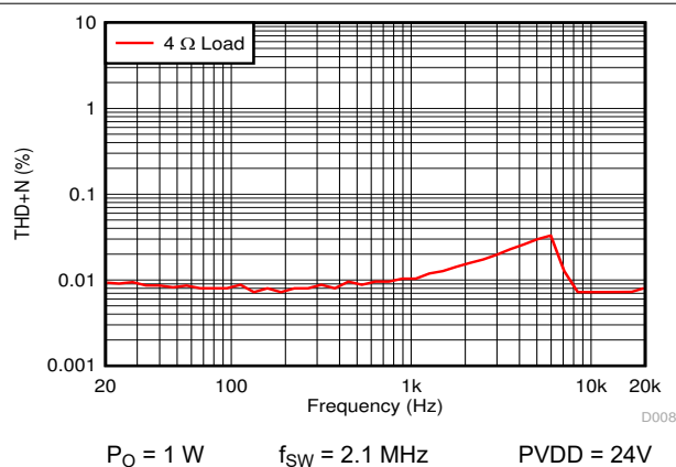
Figure 7-7. THD+N vs Frequency
