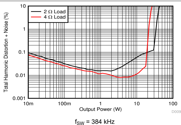
Figure 7-8. THD+N vs Power
