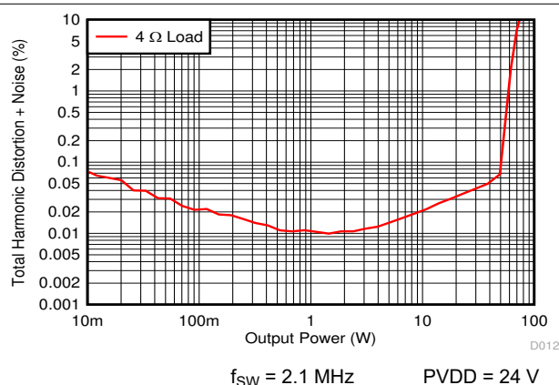
Figure 7-11. THD+N vs Power
