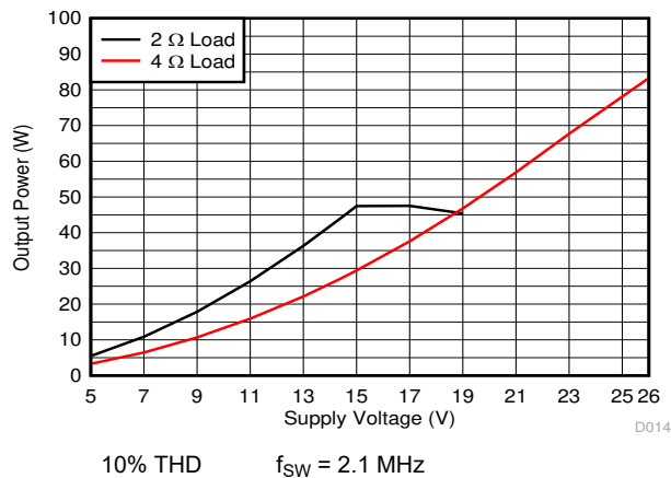
Figure 7-13. Output Power vs Supply Voltage
