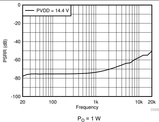
Figure 7-3. VBAT + PVDD PSRR vs Frequency
