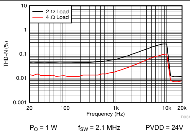
Figure 7-25. PBTL THD+N vs Frequency
