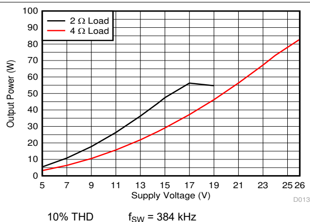
Figure 7-12. Output Power vs Supply Voltage
