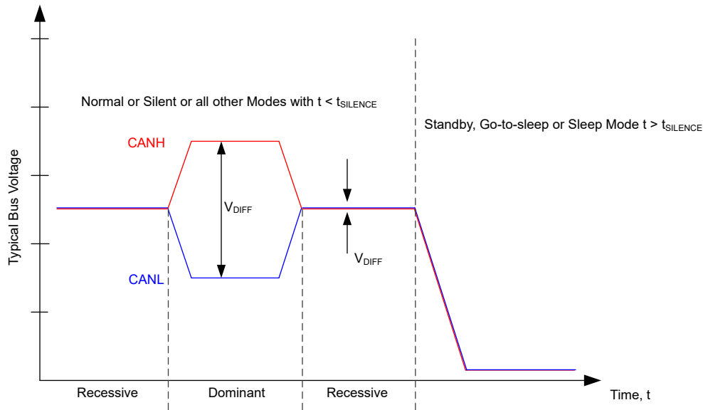
Figure 7-11. Bus States
