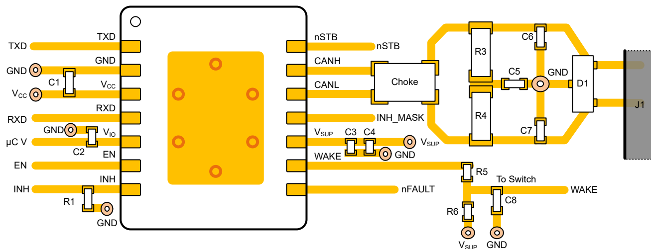
Figure 8-5. Example Layout
