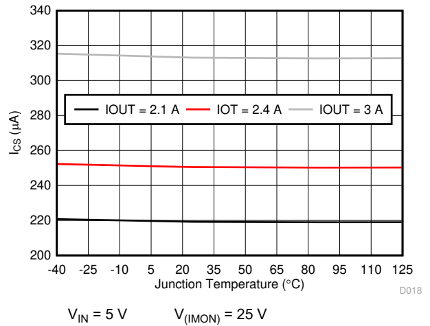
Figure 6-14. I_{(IMON)} vs Temperature
