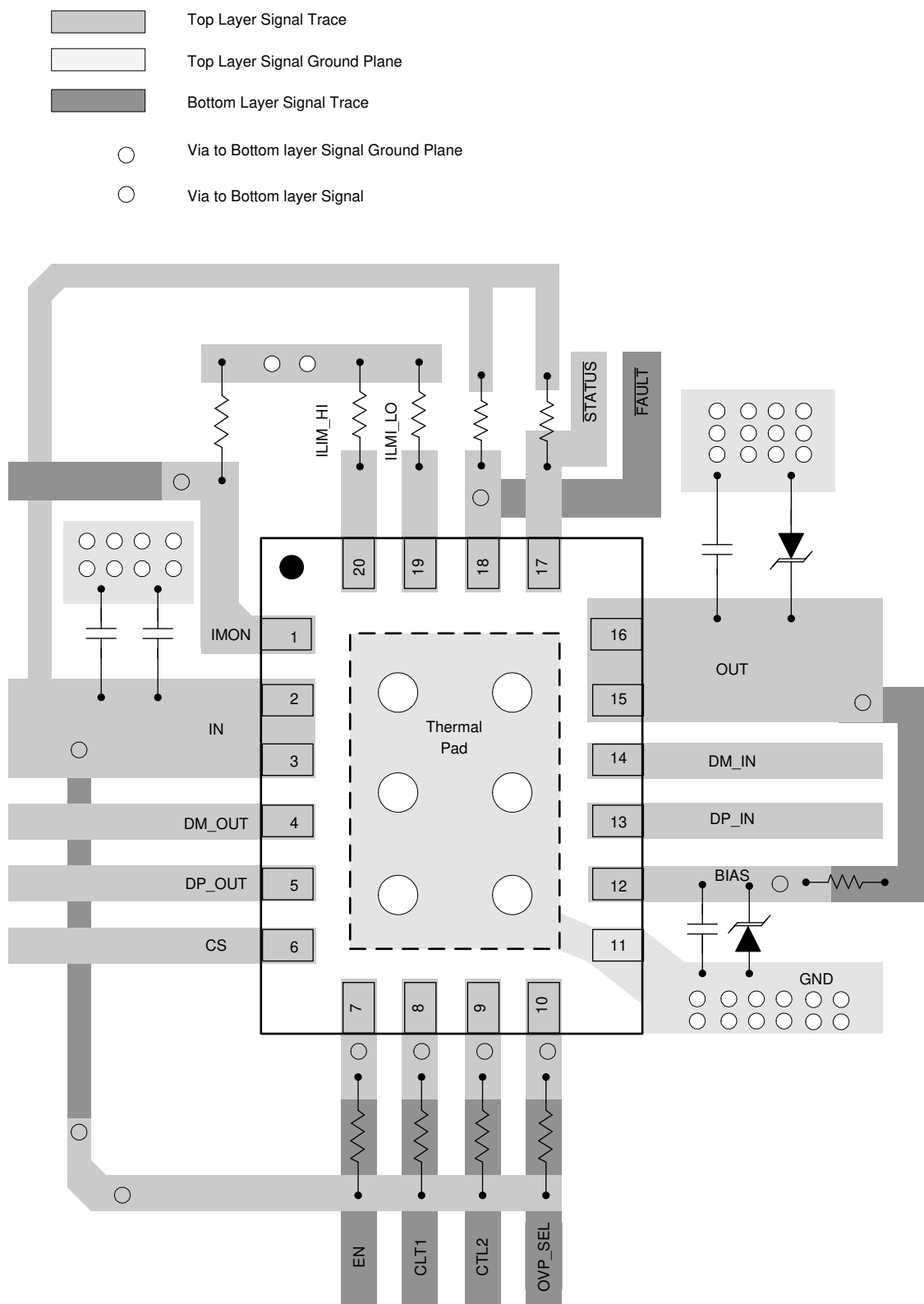
Figure 11-1. TPS254900A-Q1 Layout Diagram
