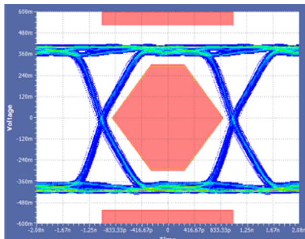
Figure 6-17. Through the TPS254900A-Q1 Data Switch
