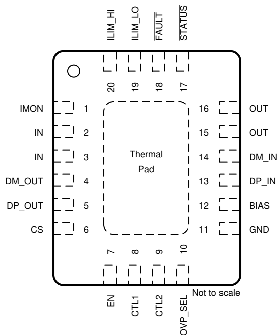
Figure 5-1. RVC Package 20-Pin WQFN Top View
