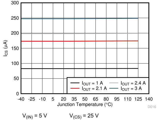
Figure 6-12. I_{(CS)} vs Temperature
