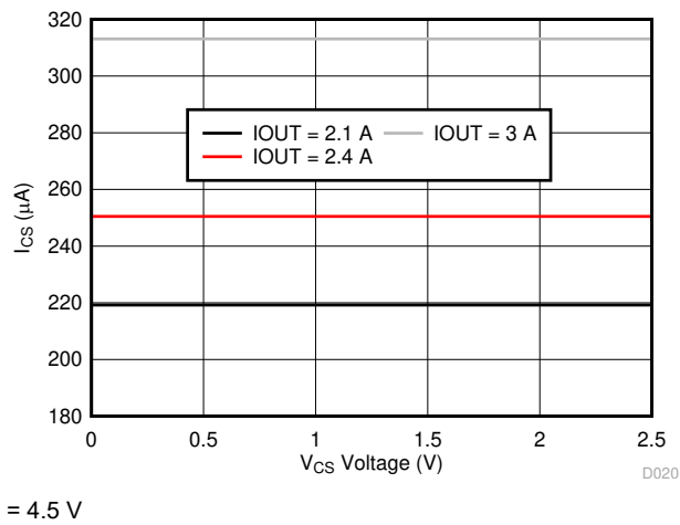
Figure 6-15. I_{(IMON)} vs V_{(CS)} Voltage
