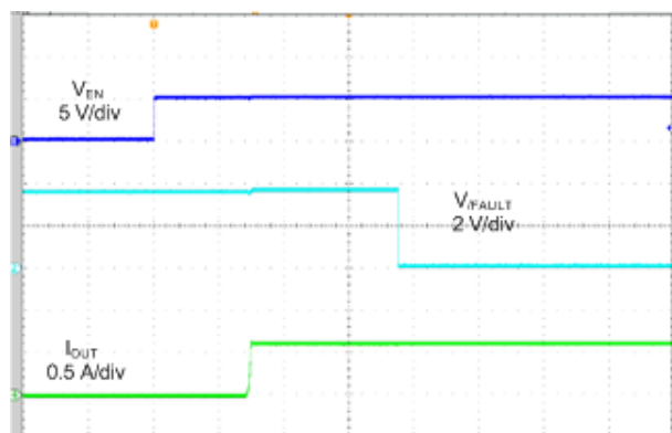
Figure 6-18. Turnon Response
