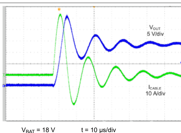
Figure 9-3. Disabled, 35-V, 1210, X7R C_{OUT} Capacitor Without SMAJ18
