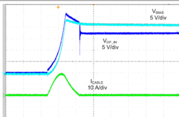
Figure 9-7. Enabled With OVP_SEL = High, OUT Shorted to Battery
