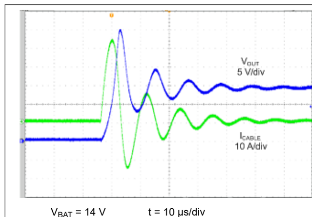
Figure 9-2. Disabled, 25-V, 1206, X7R C_{OUT} Capacitor Without SMAJ18
