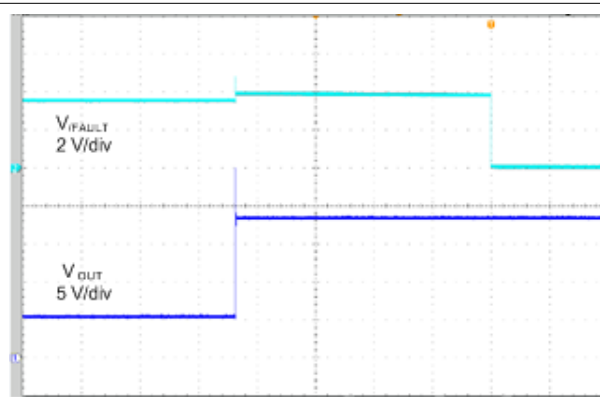
Figure 6-25. Load-Detection Set Time
