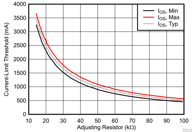
Figure 8-4. Current-Limit Setting vs Adjusting Resistor I
