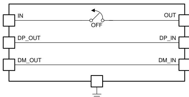
Figure 8-6. Client-Mode Equivalent Circuit
