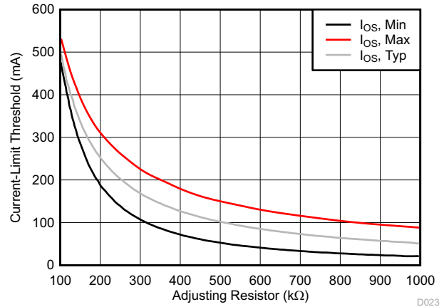
Figure 8-5. Current-Limit Setting vs Adjusting Resistor II
