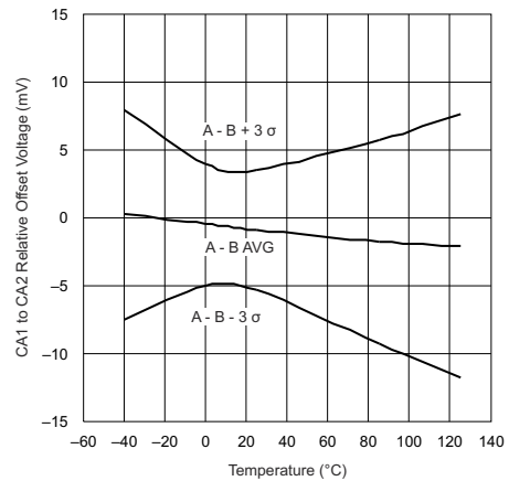
Figure 5-15. CA1 to CA2 Relative Offset vs Junction Temperature
