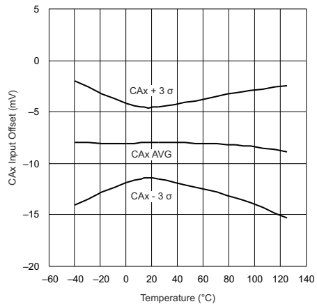
Figure 5-14. CAx Input Offset Voltage vs Junction Temperature
