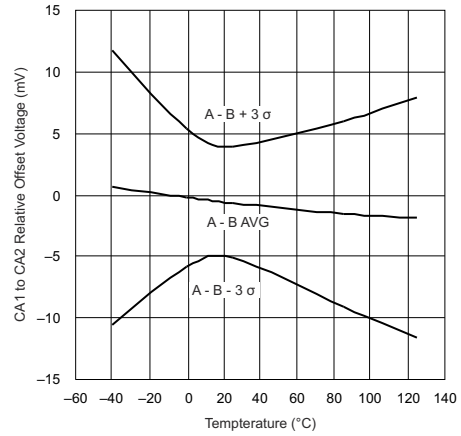
Figure 5-13. CA1 to CA2 Relative Offset vs Junction Temperature
