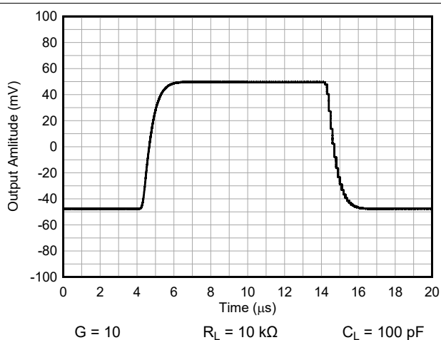
Figure 7-30. Small-Signal Response
