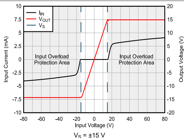
Figure 7-38. Input Current vs Input Overvoltage
