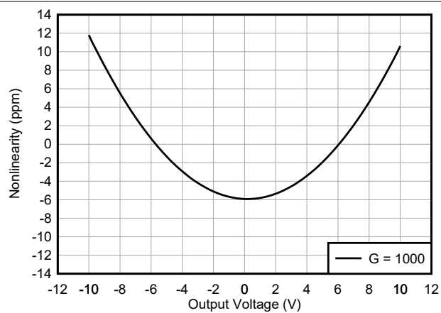
Figure 7-40. Gain Nonlinearity
