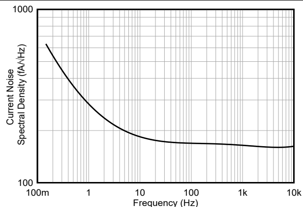
Figure 7-26. Current Noise Spectral Density vs Frequency (RTI)
