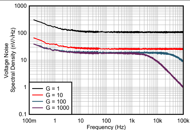
Figure 7-25. Voltage Noise Spectral Density vs Frequency (RTI)
