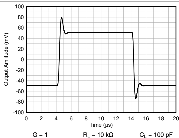
Figure 7-29. Small-Signal Response
