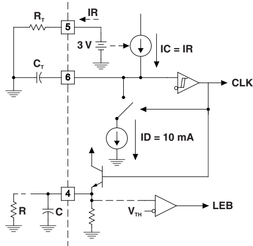
Figure 1. Oscillator
