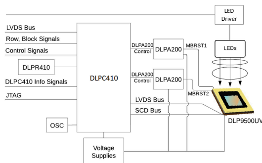
Simplified Schematic
