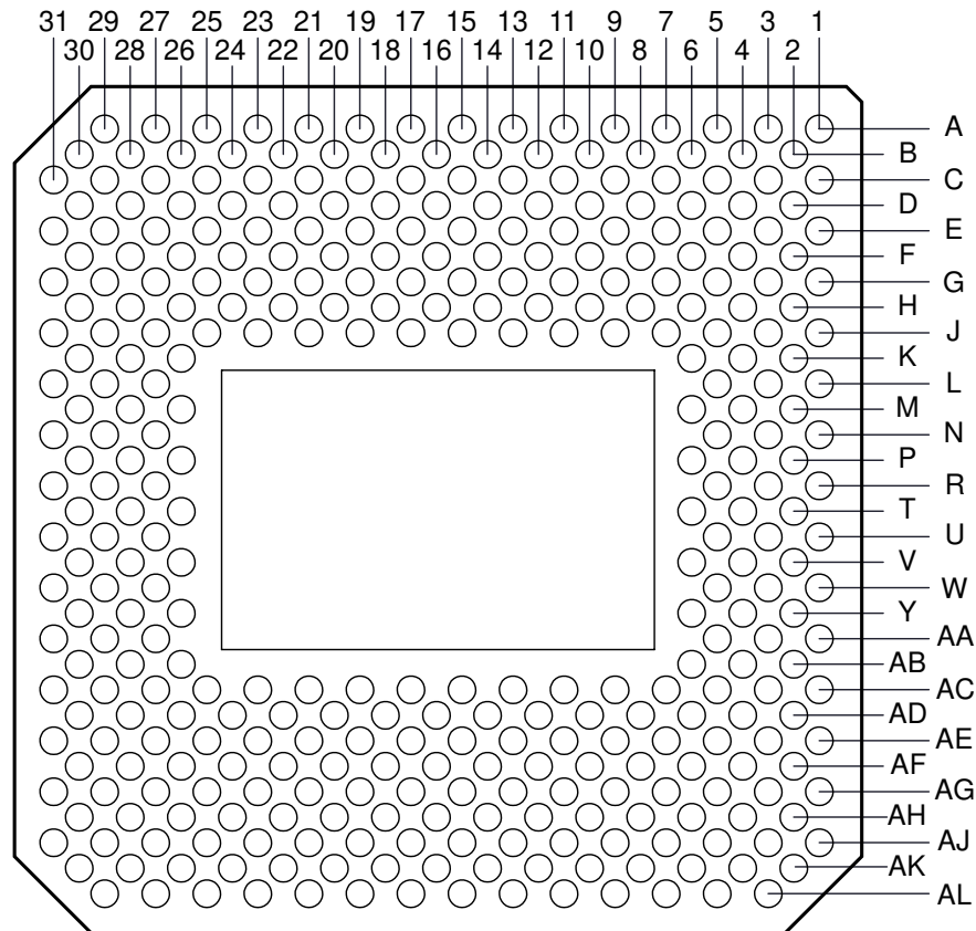
Figure 5-1. FLN Package 355-Pin LCCC Bottom View
