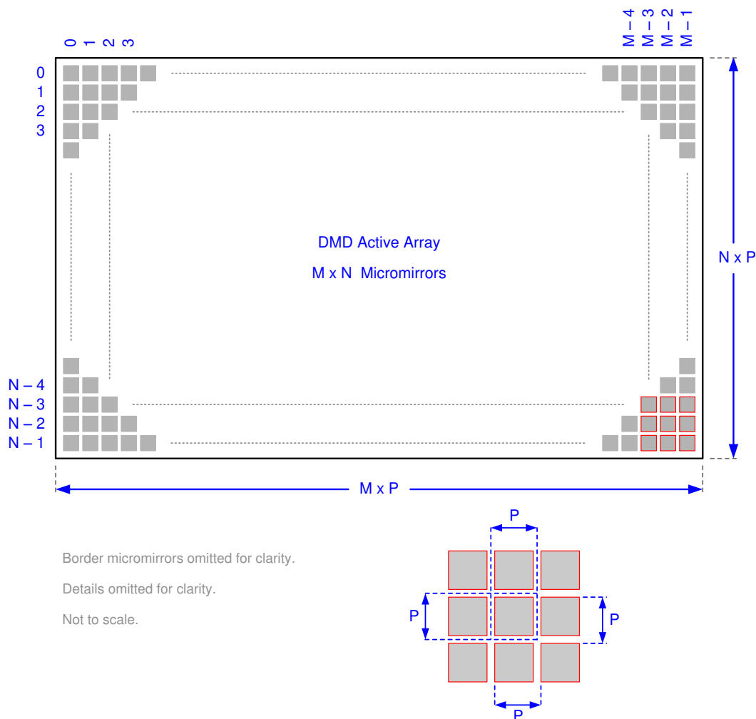
Figure 6-6. Micromirror Array Physical Characteristics
