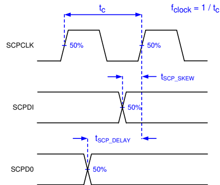
Figure 6-3. Serial Communications Bus Timing Parameters
