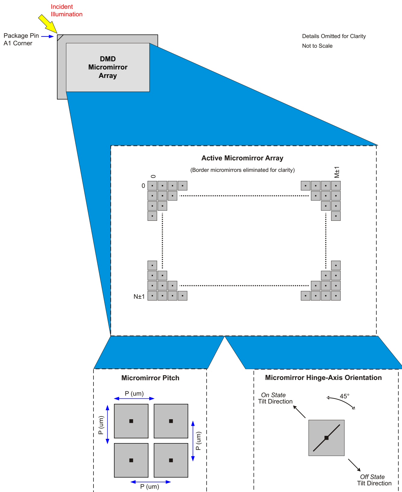
Figure 7-5. DMD Micromirror Array, Pitch, and Hinge-Axis Orientation
