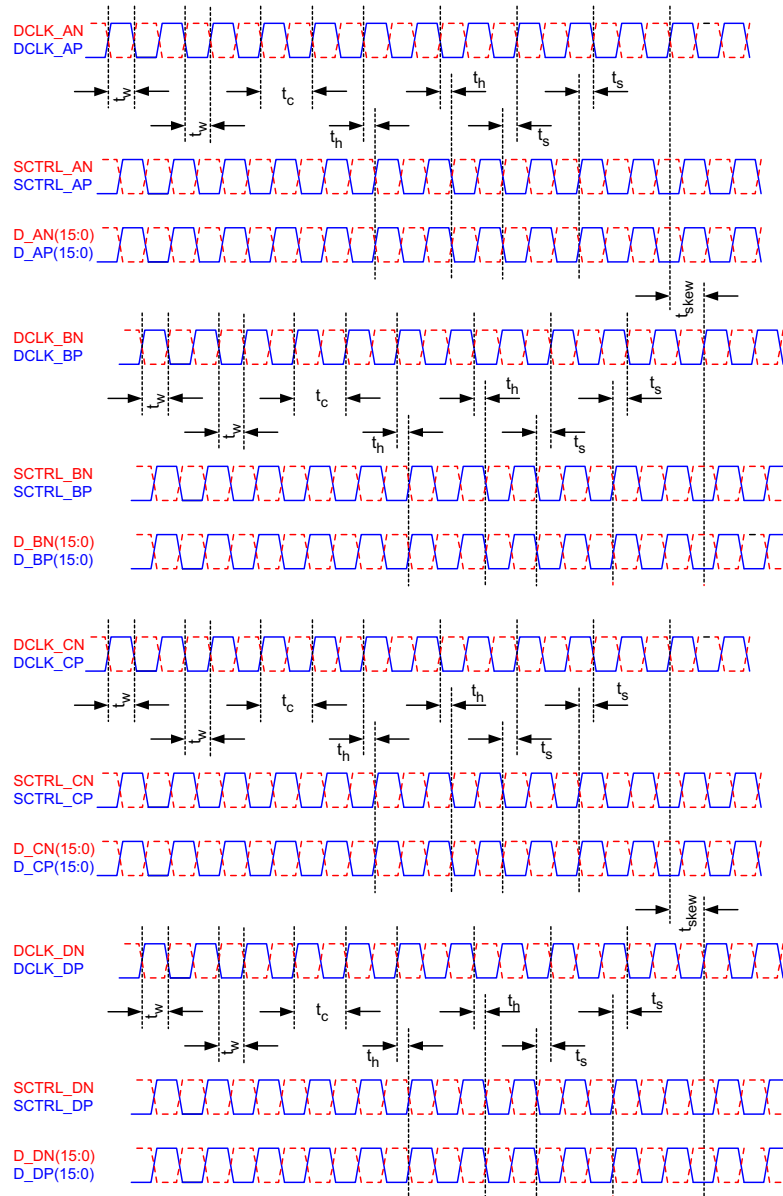
Figure 6-1. LVDS Timing Waveforms
