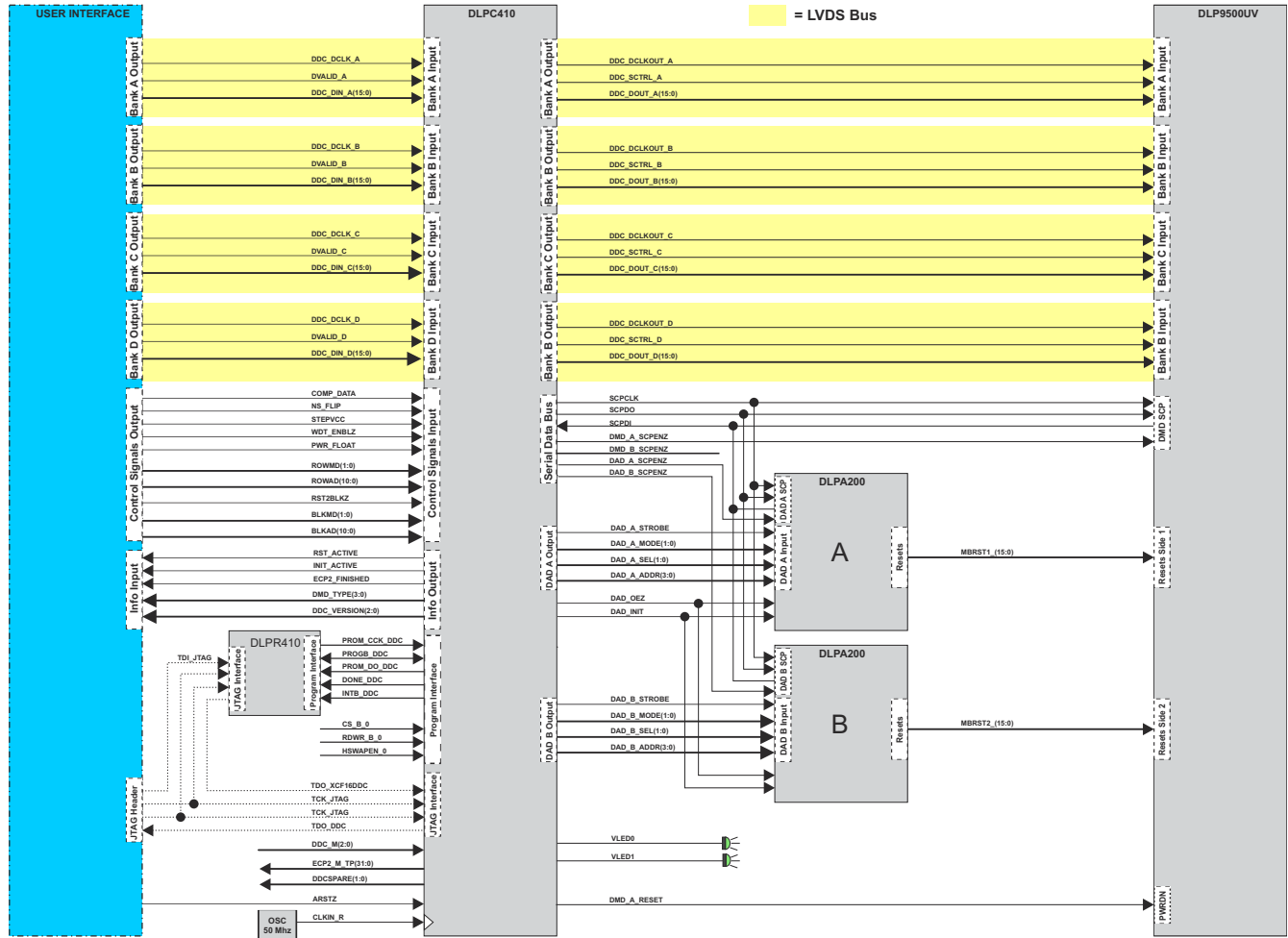
Figure 7-1. DLPC410, DLPA200, DLPR410, and DLP9500UV Functional Block Diagram
