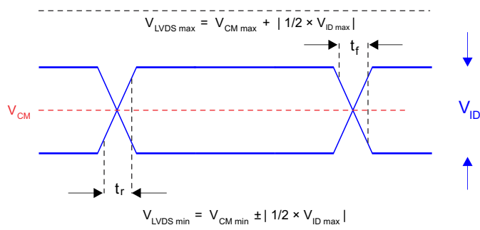
Figure 6-2. LVDS Waveform Requirements
