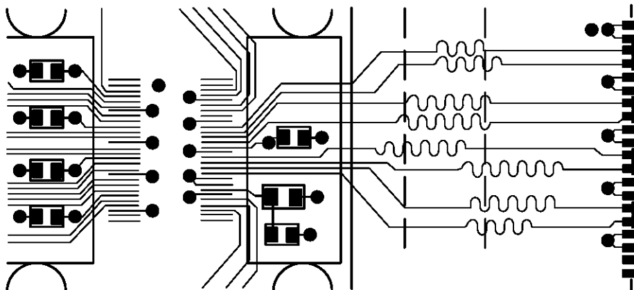
Figure 8-4. Mitering LVDS Traces to Match Lengths
