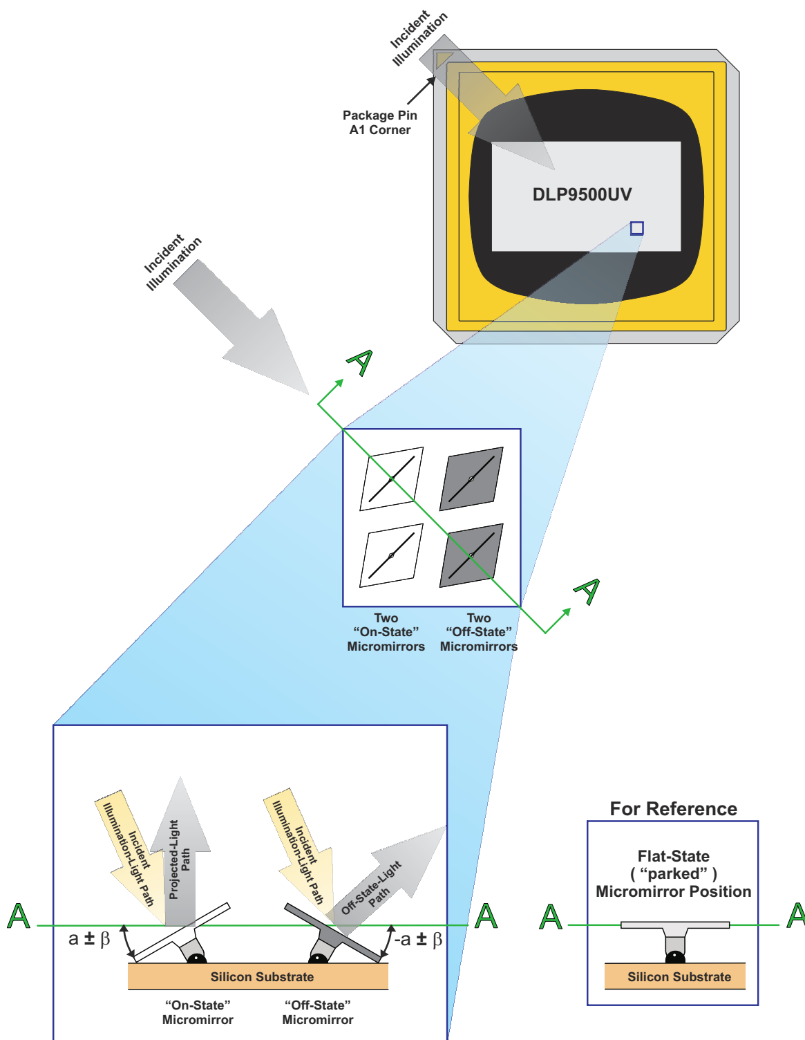
Figure 7-6. Micromirror Landed Positions and Light Paths
