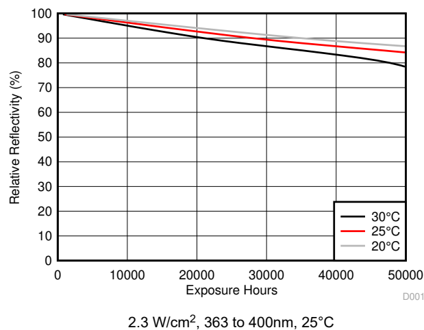
Figure 8-1. Nominal DMD Relative Reflectivity Percentage vs Total Exposure Hours
