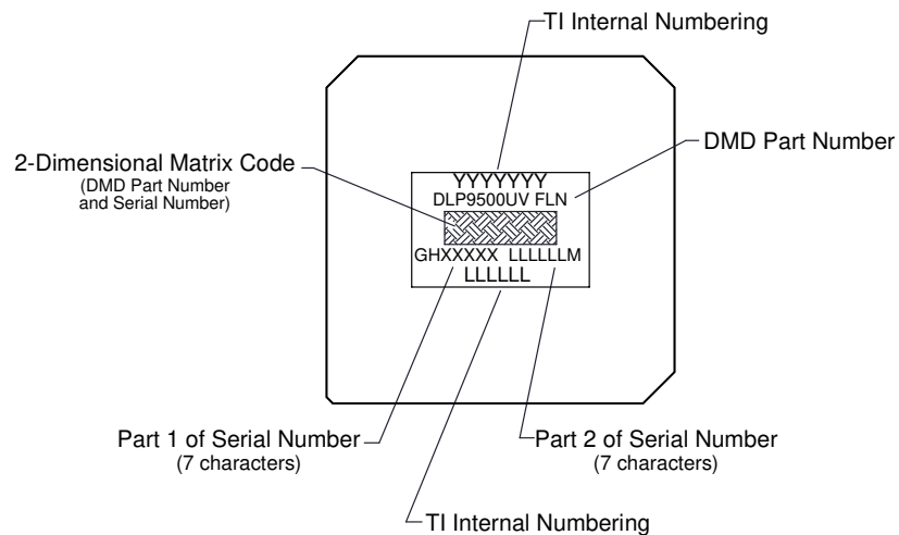
Figure 9-2. DLP9500UV Device Marking
