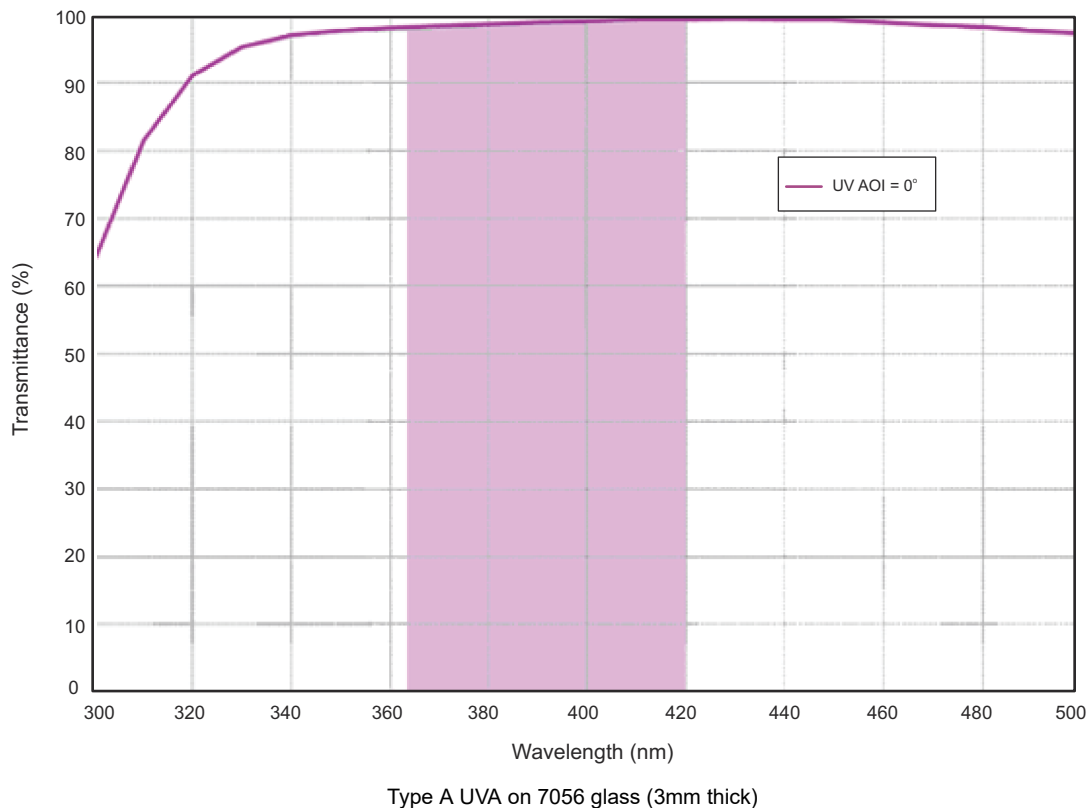
Figure 8-3. Corning 7056 UV Window Transmittance (Maximum Transmission Region)
