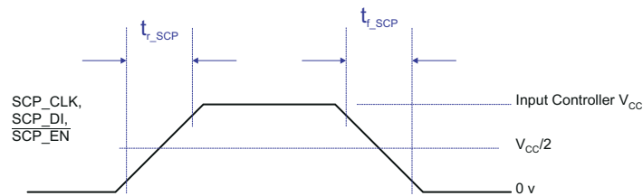
Figure 6-4. Serial Communications Bus Waveform Requirements
