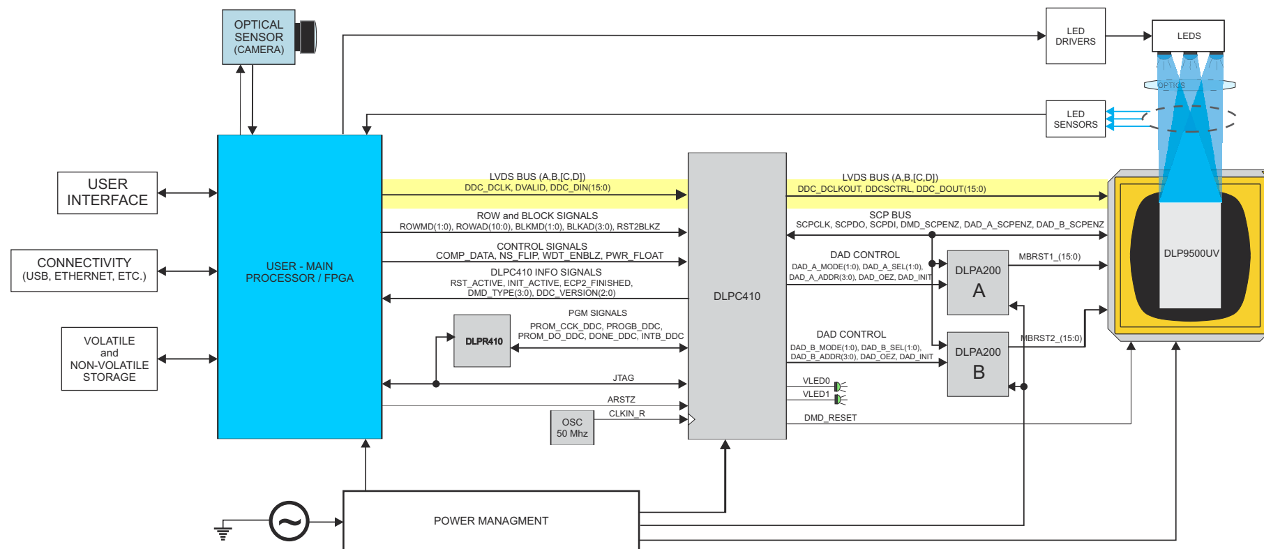
Figure 8-2. DLPC410 and DLP9500UV Embedded Example Block Diagram
