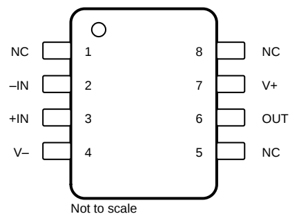
TLV379: D Package 8-Pin SOIC Top View
