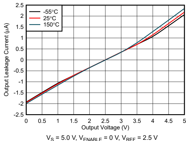
Figure 6-32. Output Leakage vs. Output Voltage (A4 and A5 Devices)
