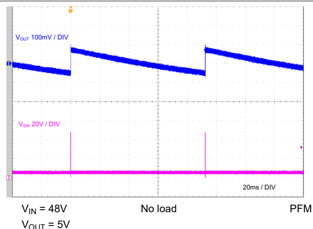
Figure 8-14. PFM Switching
