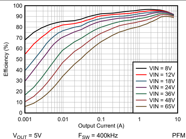
Figure 8-12. Efficiency vs I_{OUT} , Log Scale
