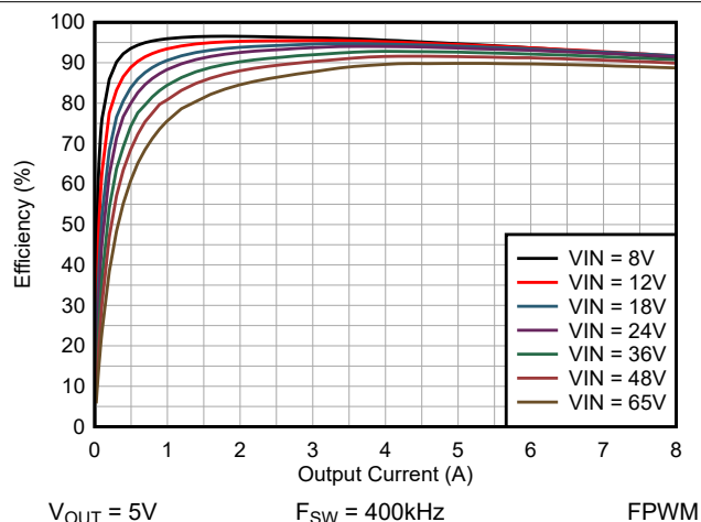
Figure 8-9. Efficiency vs I_{OUT} , Linear Scale
