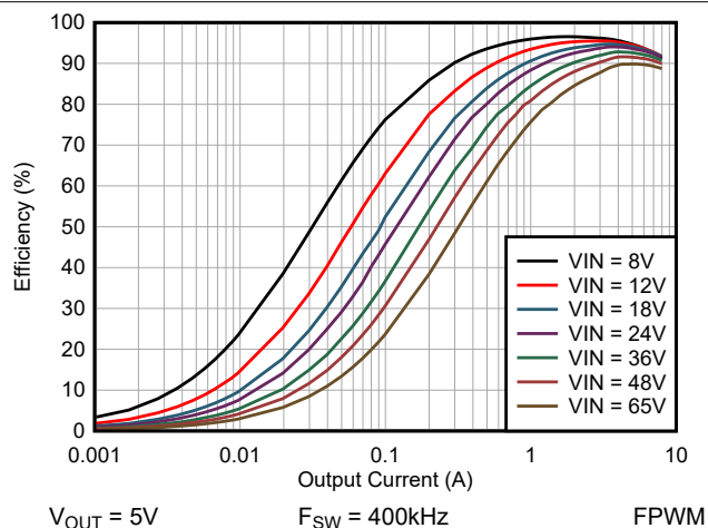
Figure 8-10. Efficiency vs I_{OUT} , Log Scale
