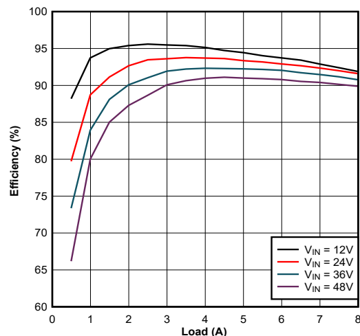
Typical Efficiency V_{OUT} = 5V , f_{SW} = 400kHz
