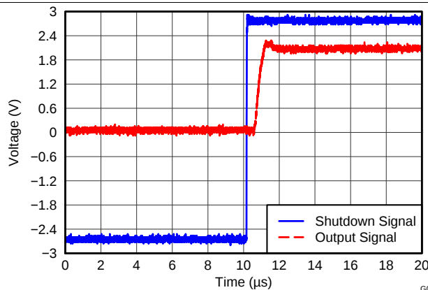
Figure 27. Turnon Transient
