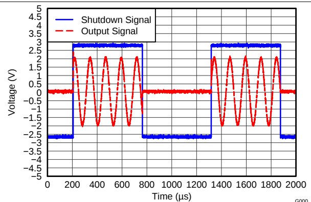
Figure 26. Turnoff Transient
