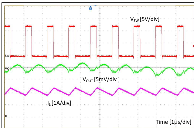
Figure 14. CCM Mode
