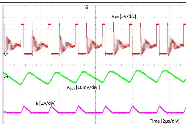
Figure 15. DCM Mode
