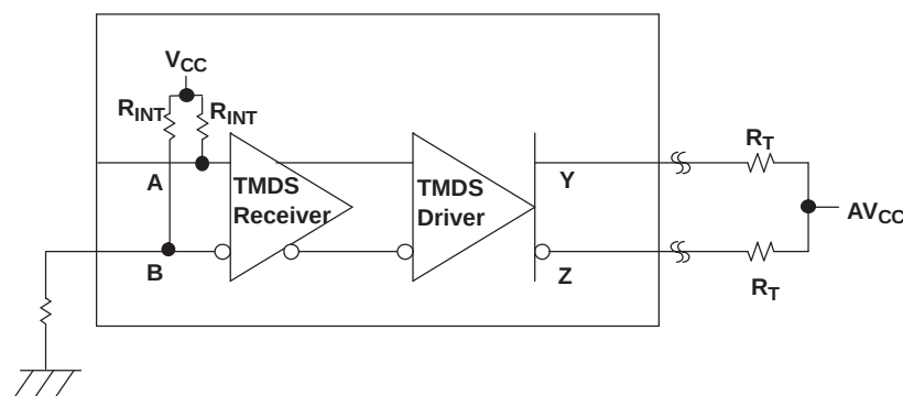
Figure 16. TMD5 Input Fail-Safe Recommendation
