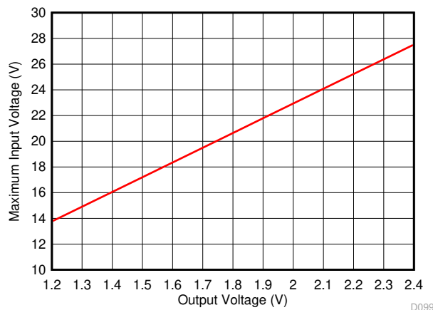
Figure 8-3. Maximum Input Voltage for V_{OUT} < 2.5\text{ V}
