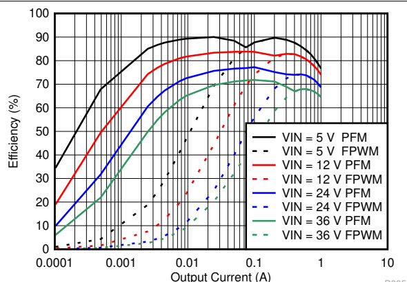
Figure 8-30. Efficiency
