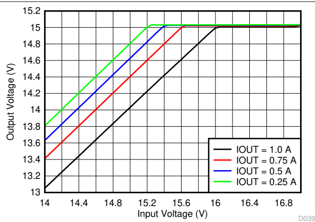
Figure 6-4. Dropout Voltage
