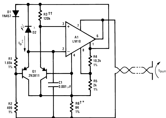
Logarithmic Light Sensor
