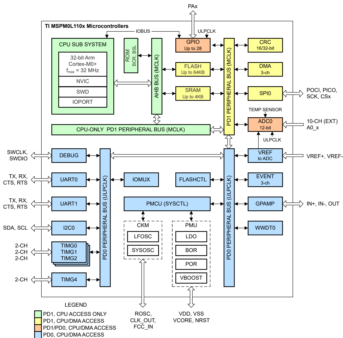
Figure 4-1. MSPM0L110x Functional Block Diagram
