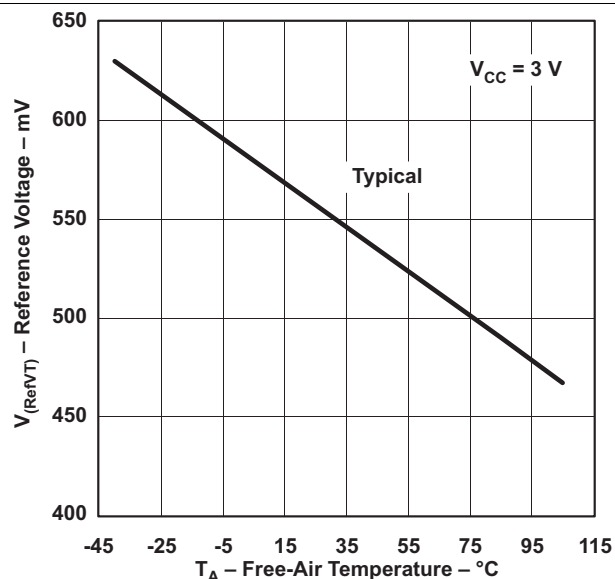
Figure 22. V (RefVT) vs Temperature, V CC = 3 V
