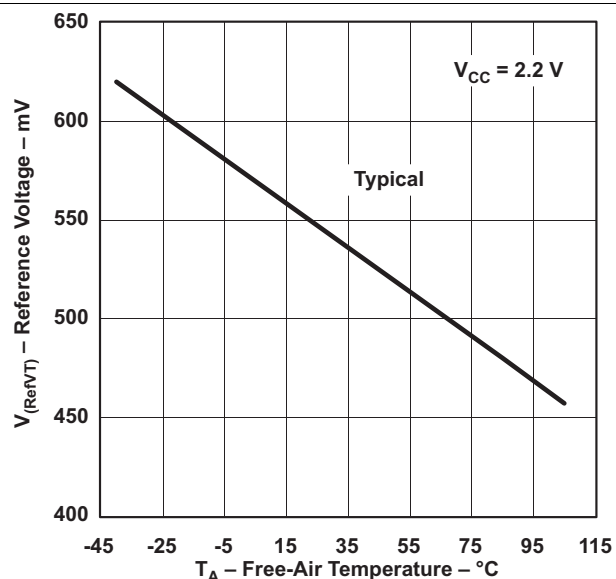
Figure 23. V (RefVT) vs Temperature, V CC = 2.2 V
