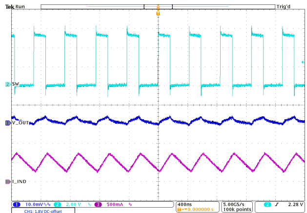
Figure 8-11. PWM Operation
