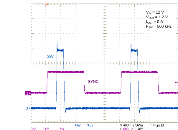
Figure 21. SYNC Waveform
