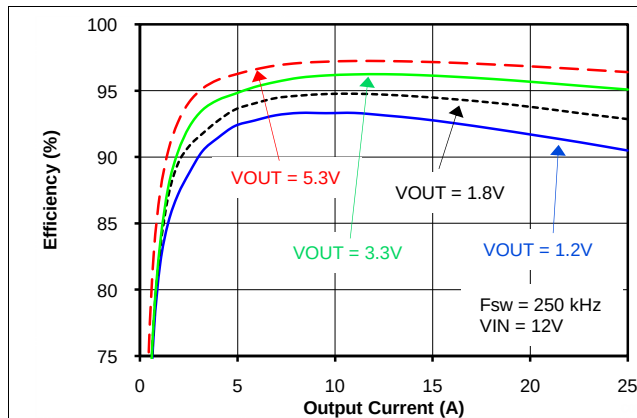
Figure 42. Efficiency vs. Output Current at V IN = 12 V
