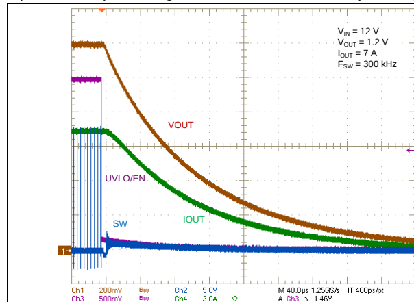
Figure 19. Shutdown Characteristic
