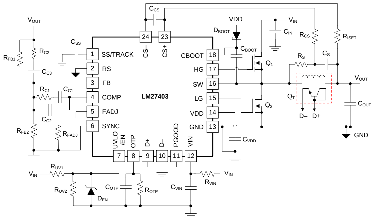
Figure 23 shows the schematic diagram for an input voltage ranging from 3 V to 20 V. Note that a finite subregulator dropout voltage exists and is manifested to a larger extent when driving high gate charge ( Q_G ) power MOSFETs at elevated switching frequencies. For example, at V_{IN} = 3 V, the VDD rail voltage is 2.8 V with a dc operating current, I_{VDD} , of 40 mA. Such a low gate drive rail may be insufficient to fully enhance the power MOSFET gates. At the very least, MOSFET on-state resistance, R_{DS(ON)} , increases at such low gate drive levels. Here are the main concerns when operating at a low input voltage:
