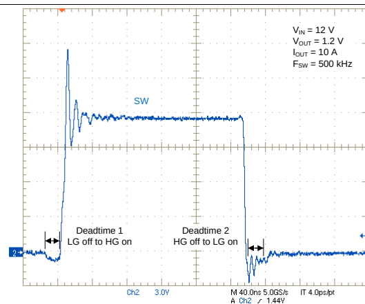
Figure 22. Switch Node Waveform
