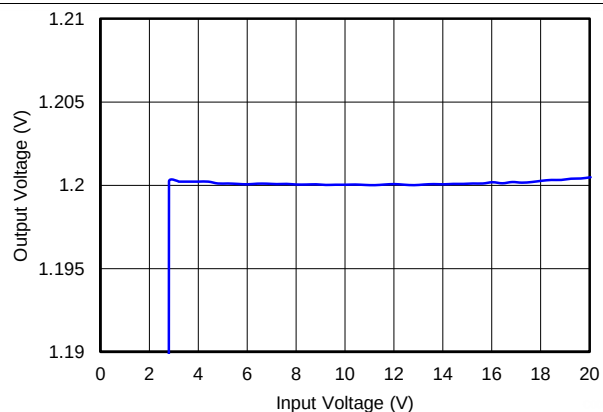
Figure 4. Line Regulation
