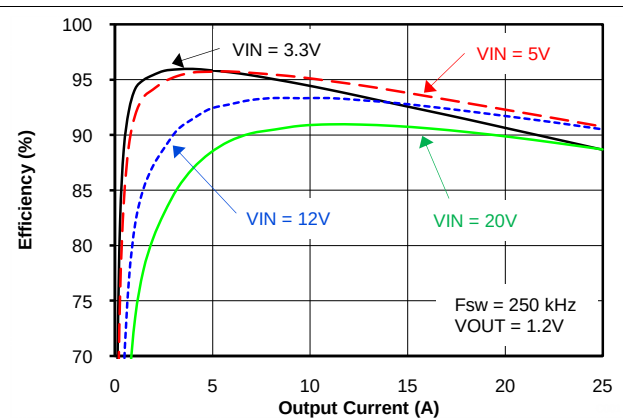
Figure 43. Efficiency vs. Output Current at V OUT = 1.2 V
