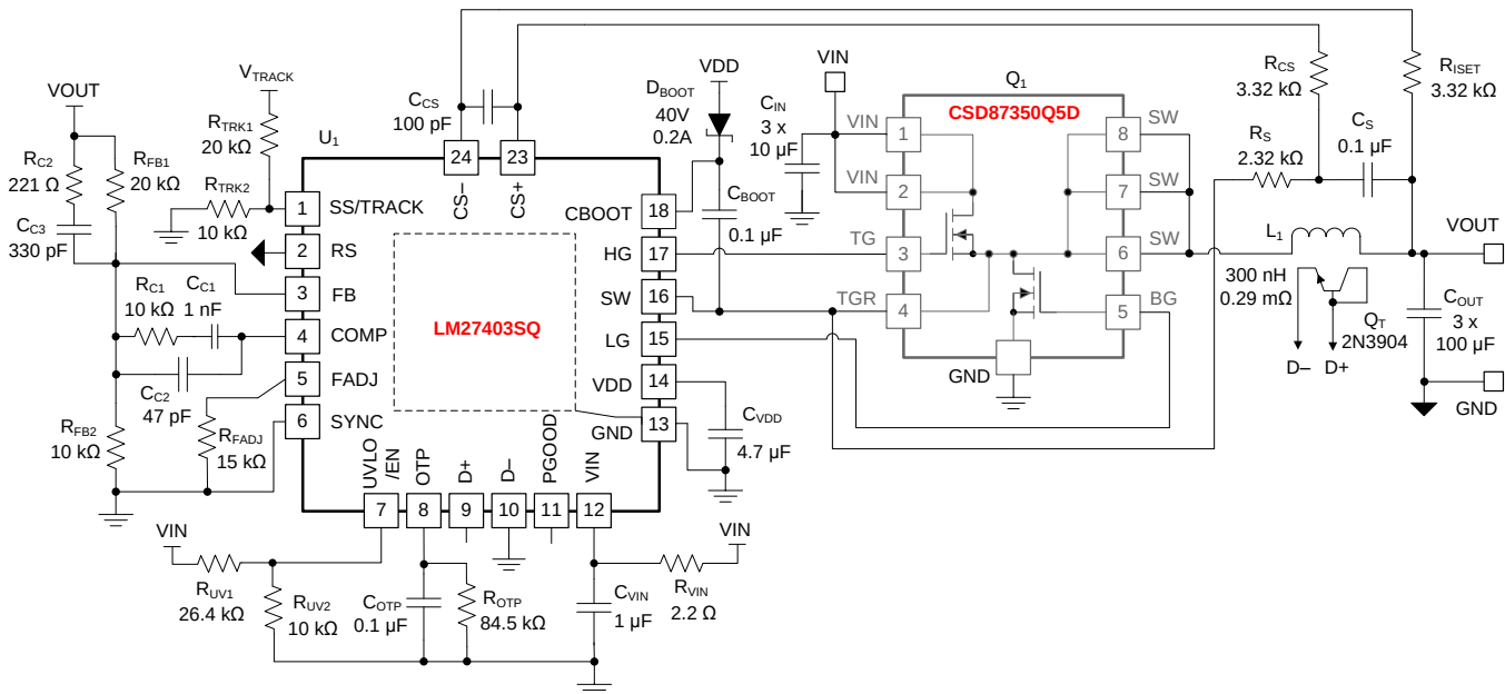
Figure 46. Application Circuit 2 With V_{IN} = 4.5\text{ V to }15\text{ V} ( V_{IN(nom)} = 12\text{ V} ), V_{OUT} = 1.8\text{ V} , I_{OUT(max)} = 30\text{ A} , F_{SW} = 600\text{ kHz}
