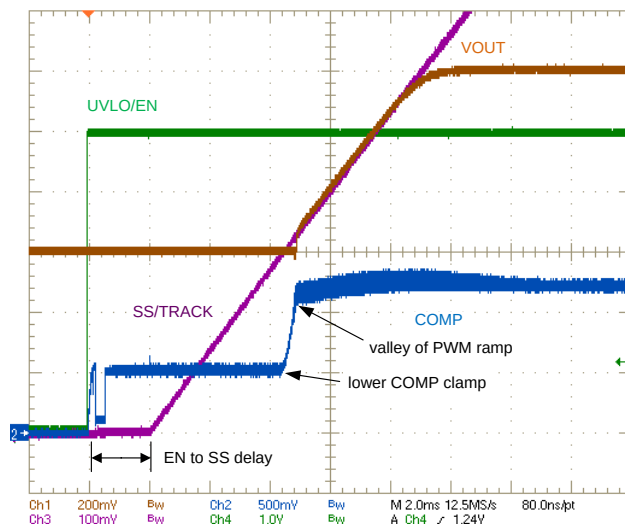
Figure 36. Typical Startup Waveforms With 0.6-V Prebiased Output, 1.2-V Nominal Output
