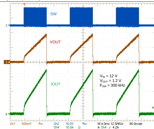
Figure 20. Current Limit Hiccup Mode
