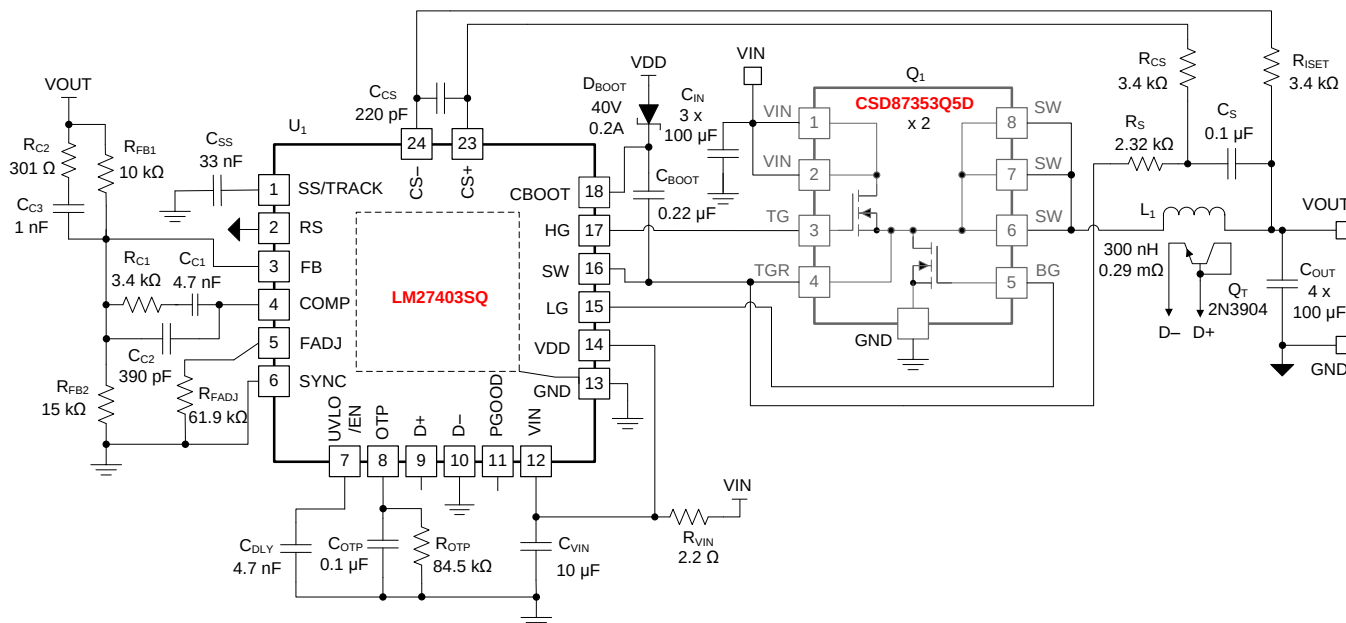
Figure 50. Application Circuit 5 With V_{IN} = 3.3\text{ V} to 5.5\text{ V} , V_{OUT} = 1\text{ V} , I_{OUT(max)} = 25\text{ A} , F_{SW} = 250\text{ kHz}
