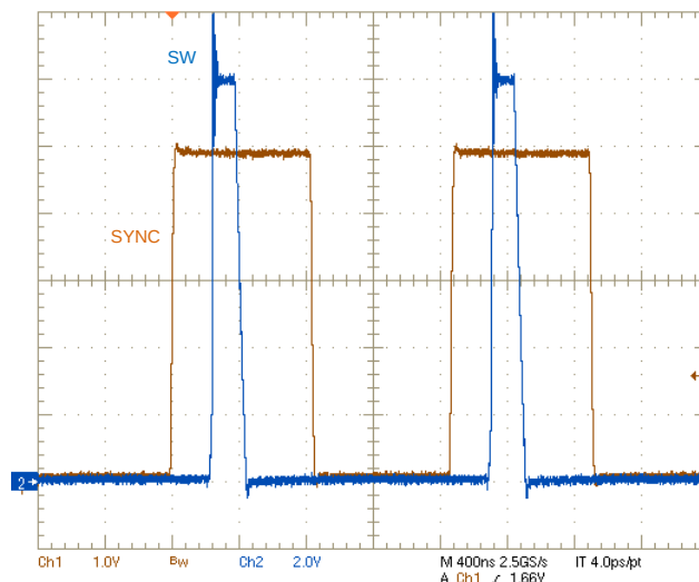
Figure 28. Typical 600-kHz SYNC Waveform
