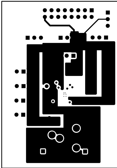
Figure 43. Layer 2
