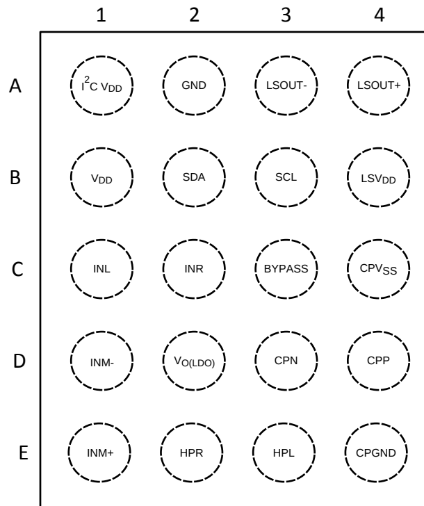
Figure 2. 20 Bump DSBGA Package - Top View (Bump Side Down) See Package Number YZR0020KGA
