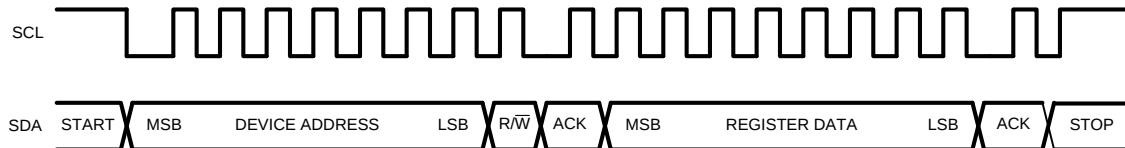
Figure 39. Start and Stop Diagram
