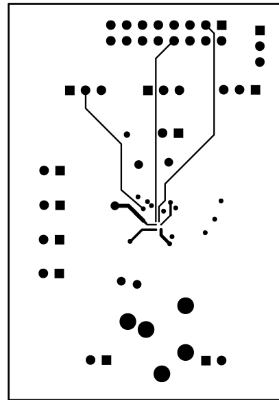
Figure 44. Layer 3
