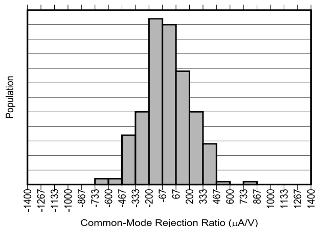
Figure 5-3. INA790B Common-Mode Rejection Production Distribution
