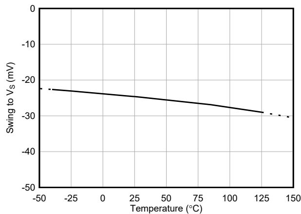
Figure 5-17. Output Voltage Swing High vs Temperature
