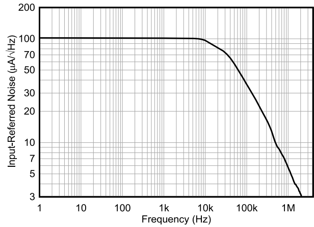
Figure 5-26. INA790A Input-Referred Current Noise vs Frequency
