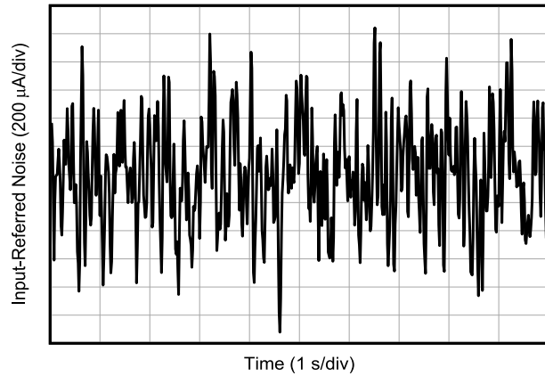
Figure 5-27. 0.1Hz to 10Hz Input-Referred Current Noise
