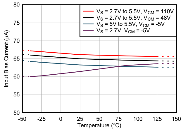
Figure 5-21. Total Input Bias Current vs Temperature
