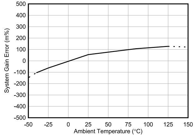
Figure 5-8. INA790B Gain Error vs Temperature
