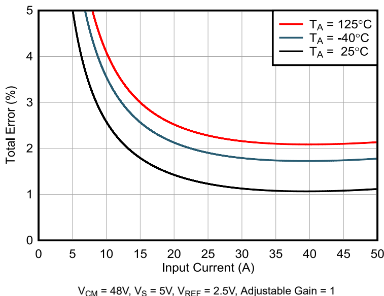
Figure 7-2. INA790B Total Error vs Input Current
