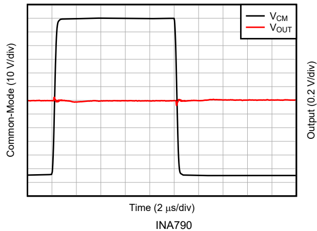
Figure 5-29. -4V to 110V Common-Mode Step Transient Response
