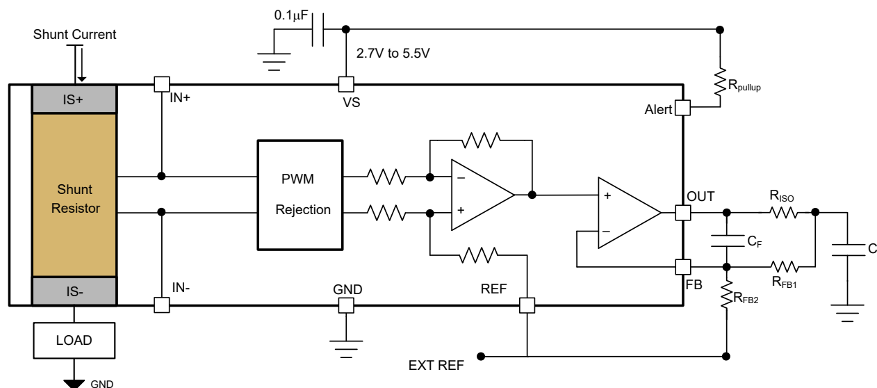
Figure 7-5. INA790x With RISO-Dual-Feedback
