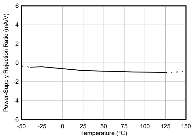
Figure 5-5. Power-Supply Rejection Ratio vs Temperature
