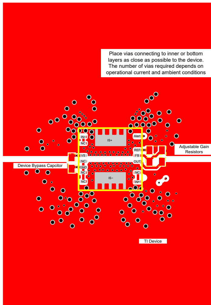
Figure 7-12. INA790x Layout Example
