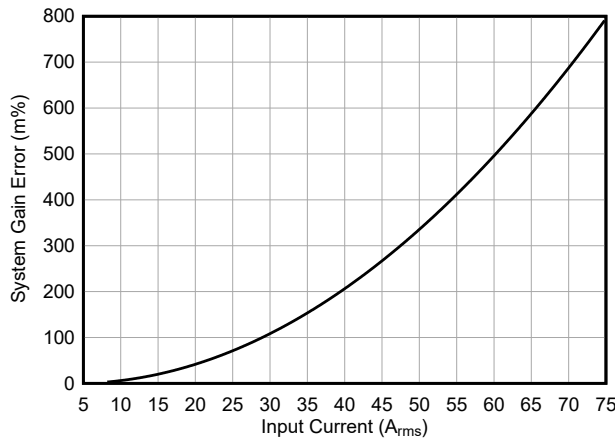
Figure 5-9. INA790B System Gain Error vs Input Current
