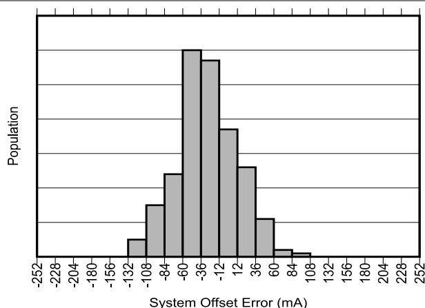
Figure 5-1. INA790B Input Offset Current Production Distribution
