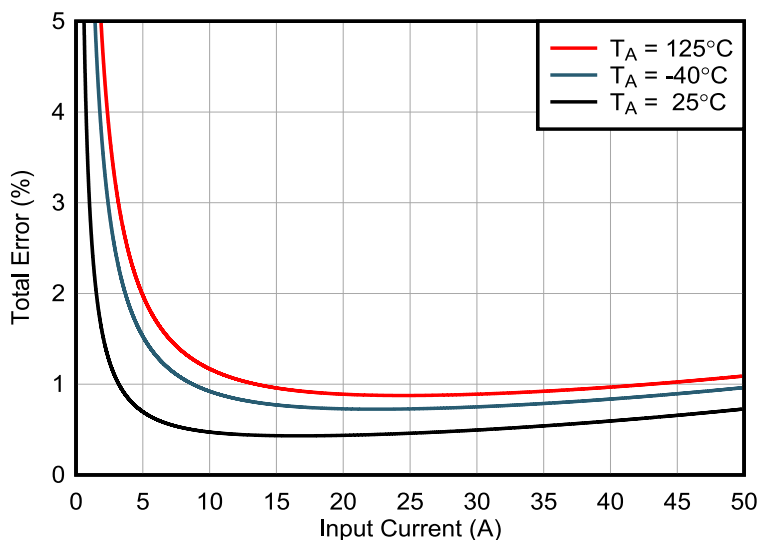
Figure 7-1. INA790A Total Error vs Input Current
