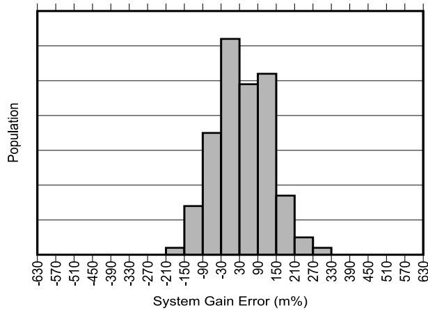
Figure 5-7. INA790B Gain Error Production Distribution
