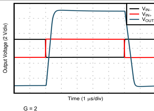
Figure 7-46. Large Signal Step Response
