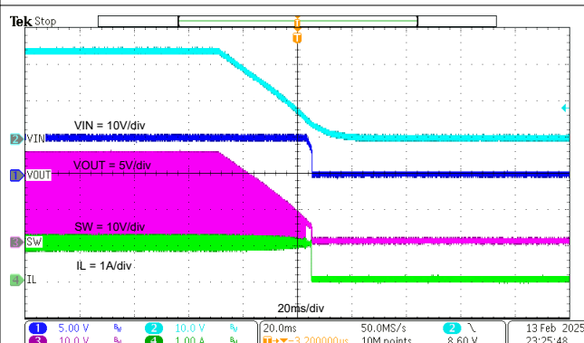
Figure 7-7. TPS561300EVM Shutdown Relative to V_{IN}
