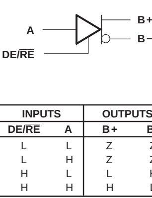
DRIVER WITH ENABLE
