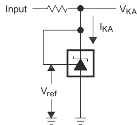
Figure 6-1. Test Circuit for V_{KA} = V_{\text{ref}}
