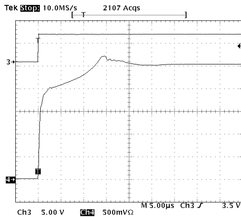
Figure 5-13. Pulse Response
