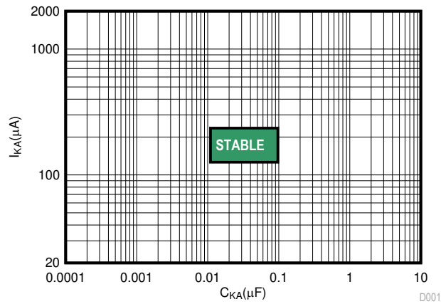
Figure 5-17. Low I_{KA} ( V_{KA} = 15.0V ) Stability Boundary Conditions All ATL43xx Devices
