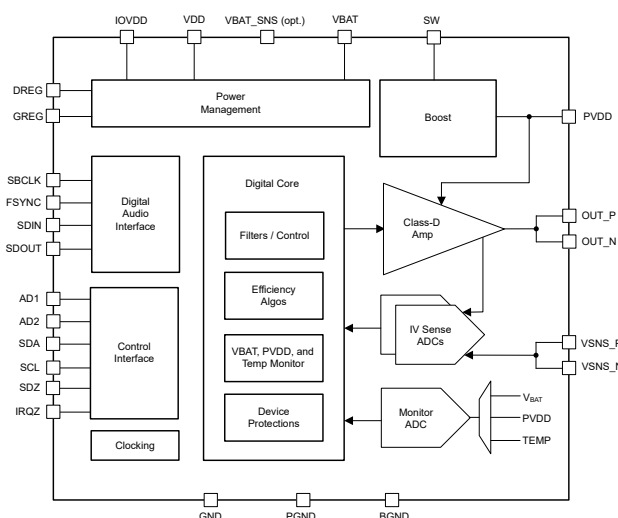
Figure 3-1. Functional block diagram
