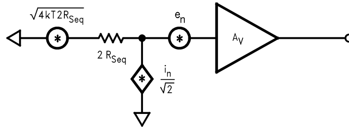
Figure 42. Noise Model with R_f \parallel R_g = R_{seq}
