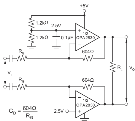
Figure 7-2. 5V Differential Configuration Test Circuit
