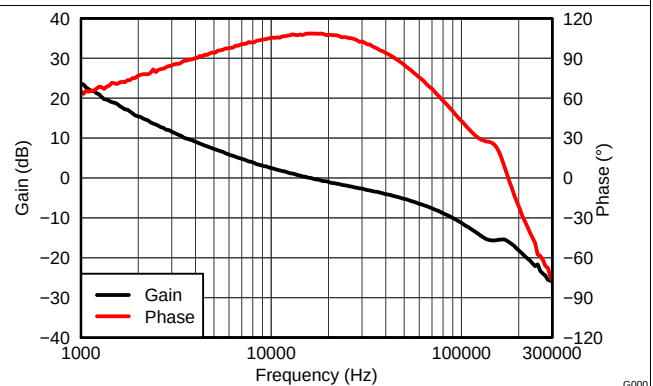
Figure 24. VOUT = 12 V, IOUT = 2 A, COUT1 = 44 µF ceramic, COUT2 = 56 µF electrolytic, fSW = 800 kHz
