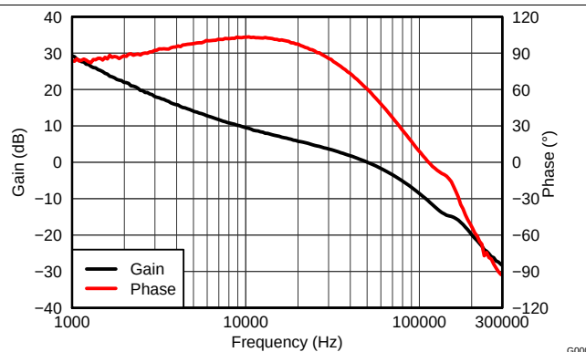
Figure 23. VOUT = 5 V, IOUT = 2 A, COUT1 = 44 µF ceramic, COUT2 = 56 µF electrolytic, fSW = 500 kHz
