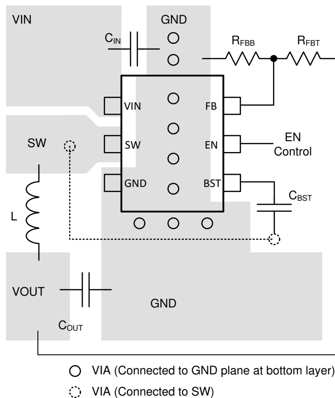
Figure 11-1. TPS563207 Layout
