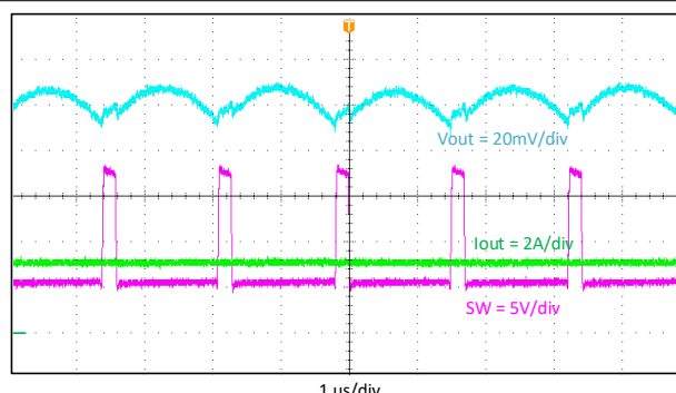
Figure 9-7. Output Voltage Ripple, Iout = 3 A
