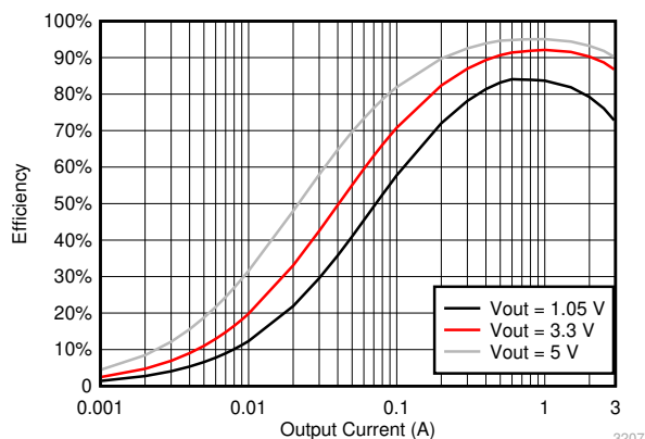
TPS563207 Efficiency
