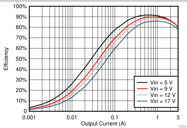
Figure 7-12. V_{OUT} = 1.8\text{-V} Efficiency, L = 2.2\text{ }\mu\text{H}
