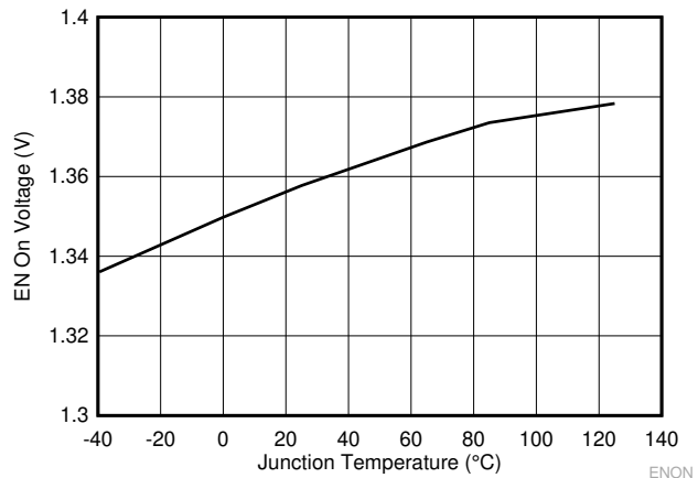
Figure 7-4. EN Pin EN On Voltage vs Junction Temperature
