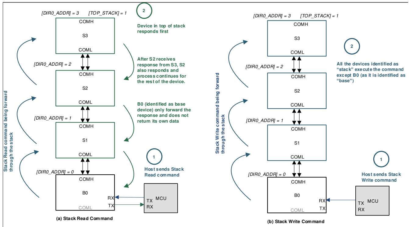
Figure 9-29. Stack Read/Write
