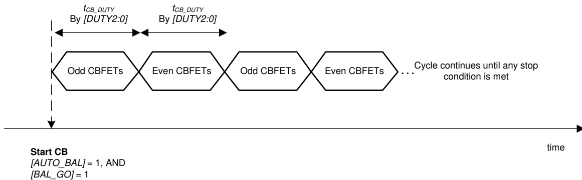
Figure 9-14. Auto Balancing Control, Example 1
