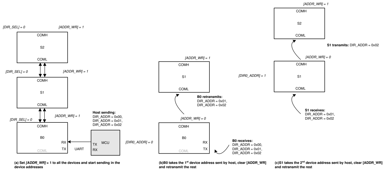
Figure 9-36. Auto-Addressing
