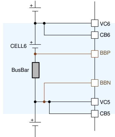
Figure 9-5. Simplified BBP and BBN Connections
