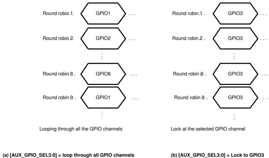
Figure 9-11. GPIO Slot with Different [AUX_GPIO_SEL3:0] Setting
