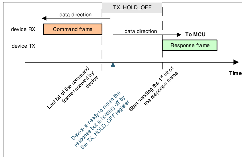
Figure 9-25. UART TX_HOLD_OFF
