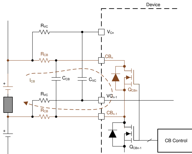
Figure 9-53. Cell Balancing with Bus Bar (Through BBP/N) Sharing a Cell Channel
