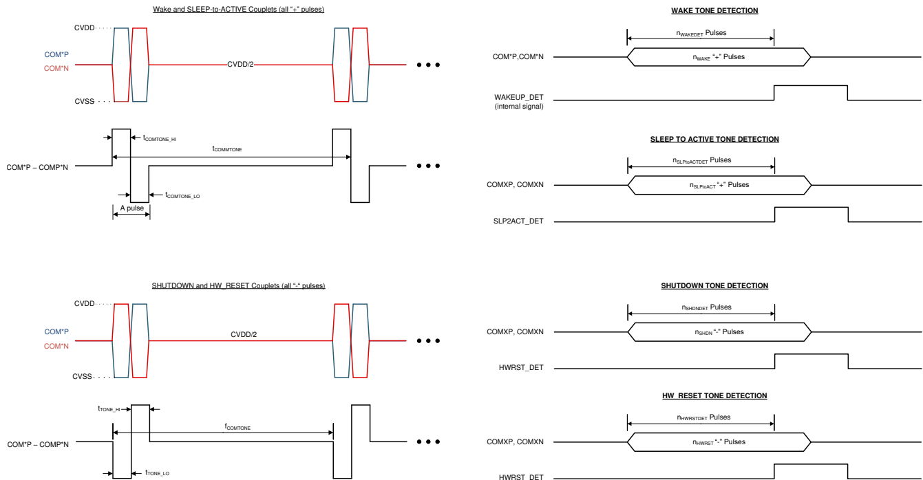
Figure 9-63. Communication Tones
