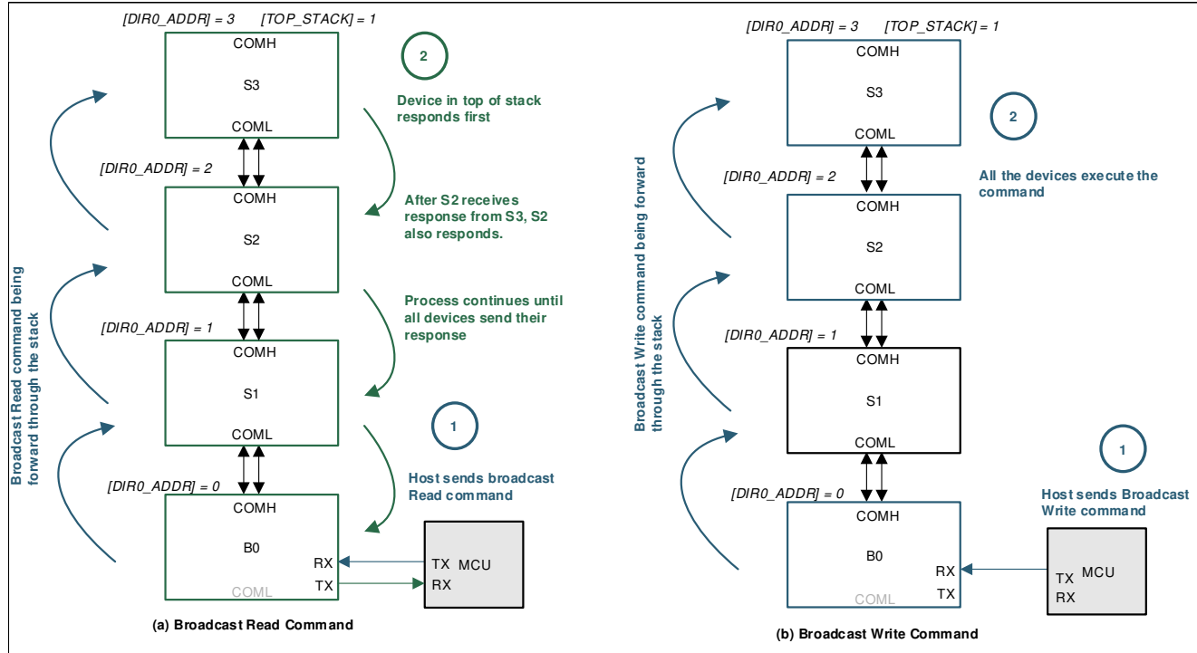
Figure 9-30. Broadcast Read/Write
