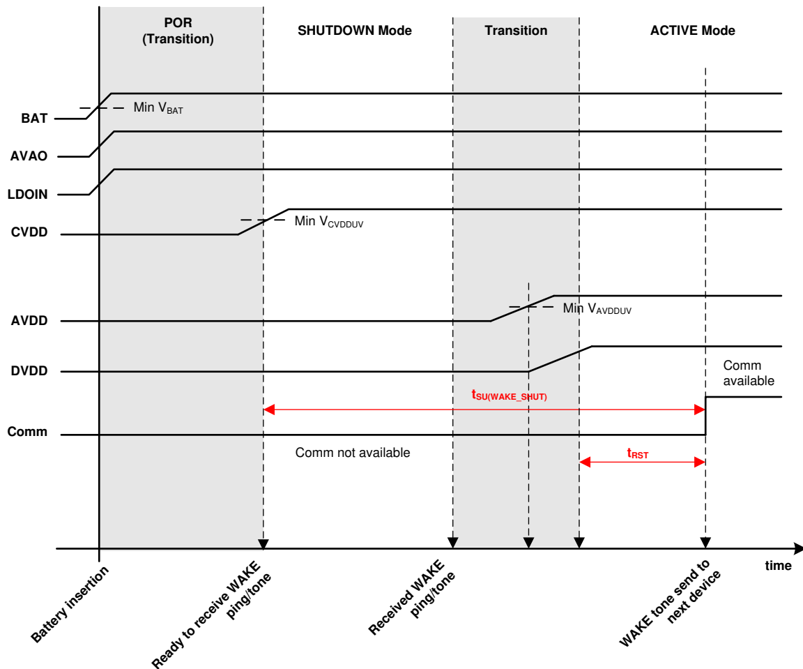
Figure 9-60. SHUTDOWN to ACTIVE Mode Transition
