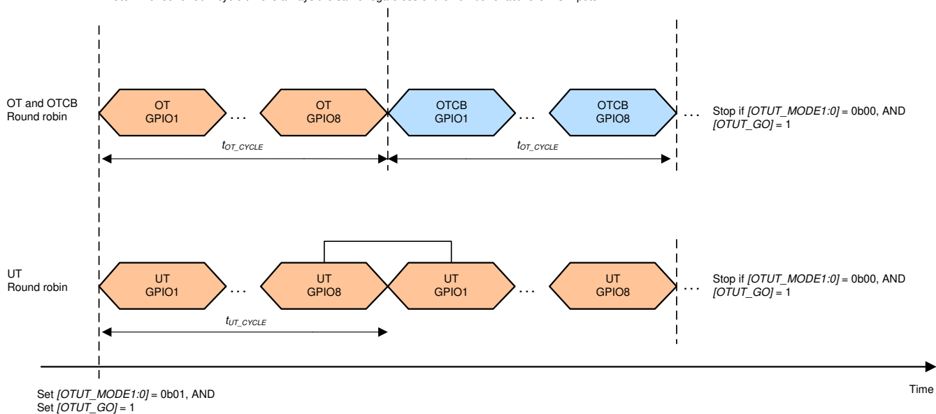
Figure 9-22. OT and UT Round Robin Modes
